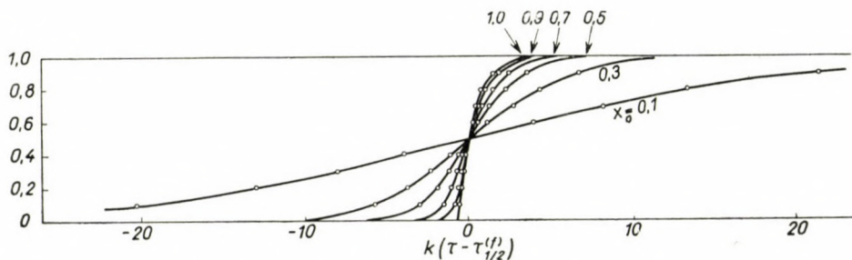
Fig. 2. Curves of the sorption front shape ( f ), for different values of x_0 , according to equ. (37)
