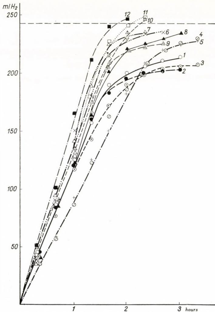
Fig. 7. Hydrogen uptake of eugenol in the presence of dimethylaniline Legend of numbers of catalysts in Table I
