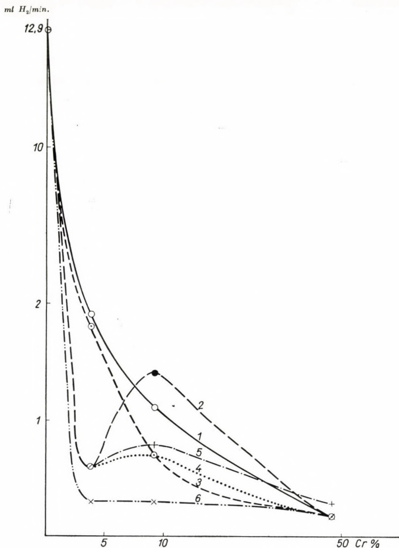
Fig. 9. Changes in activities of catalysts with various model substances, plotted against contents of chromium 1. Eugenol, 2. Acetone, 3. Acetophenone, 4. Benzophenone, 5. Benzaldehyde, 6. Benzylcyanide
