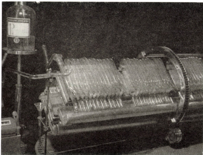
Fig. 10. Application of the aluminium trough
