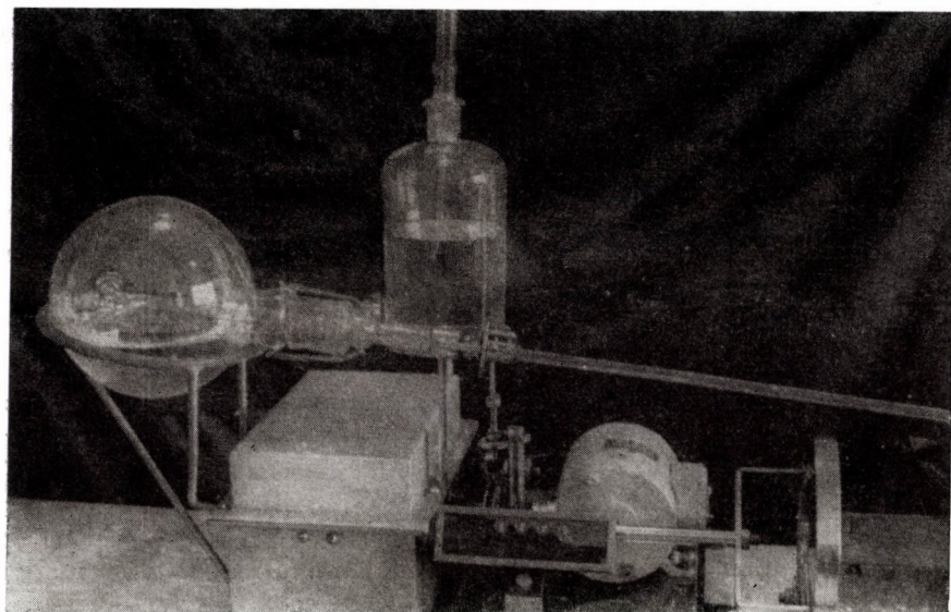
Fig. 2. Automatics for the apparatus with 50 elements
