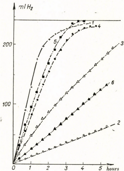
Fig. 5. Hydrogenation of benzaldehyde 1, Raney-Ni, 2, K1, 3, K2, 4, K3, 5, K4, 6, K5, 7, K6
