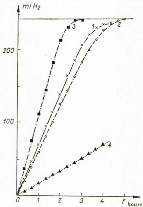
Fig. 7. Hydrogenation of acetophenone 1. Raney-Ni, 2. K4, 3. K5, 4. K6
