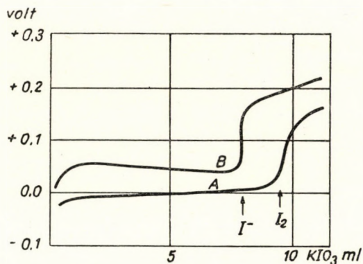
Fig. 3. Titration of 0,0487 g of antimon with a 0,1000 N solution (1/6 M) of KIO_3 . Curve A: reduction to iodine, curve B: reduction to iodide in the presence of silver chloride (1 N HCl)
