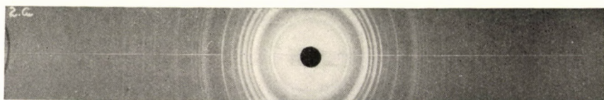
Fig. 2. Diffraction pattern of SiO_2
