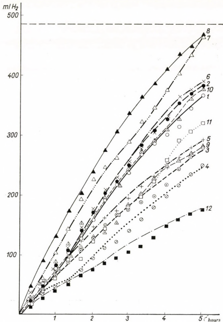
Fig. II. Hydrogen uptake of benzylcyanide in the presence of dimethylaniline Legend of numbers of catalysts in Table I
