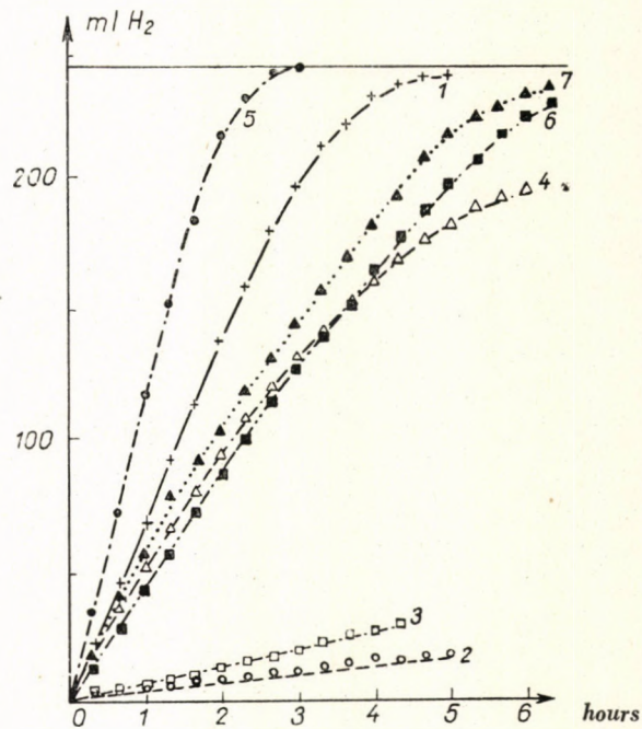
Fig. 6. Hydrogenation of acetone 1, Raney-Ni, 2, K1, 3, K2, 4, K3, 5, K4, 6, K5, 7, K6
