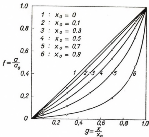
Fig. 1. Relation between a/a_0 and x/x_0 , within the steady front, for different values of x_0 , according to equ. (19)
