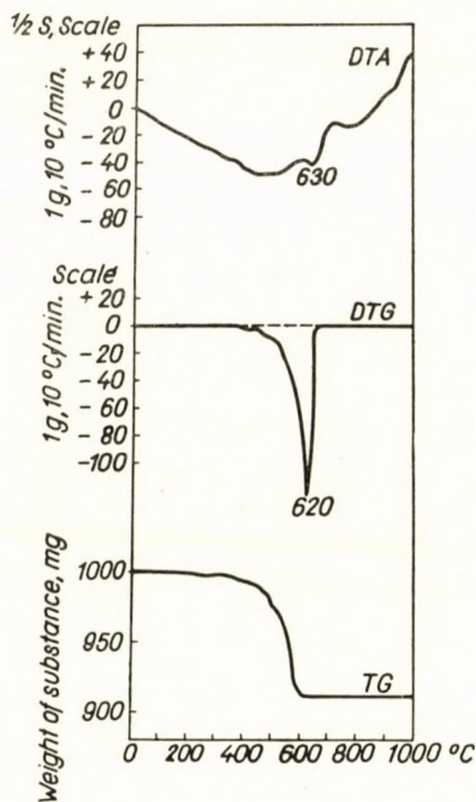
Fig. 10. Thermograms of mixture L15
