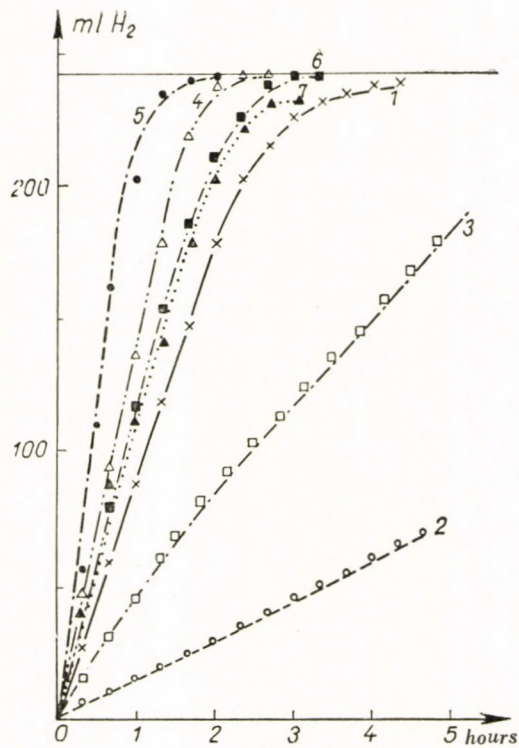
Fig. 4. Hydrogenation of cyclohexene
