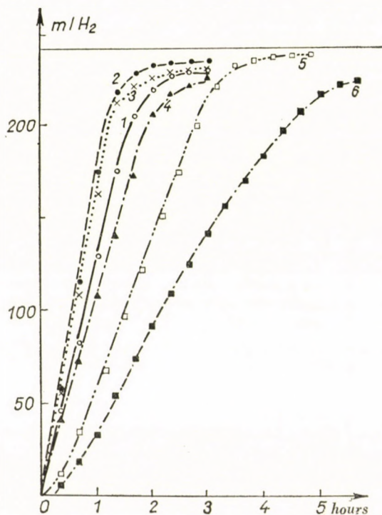
Fig. 1. Effect of temperature of reduction and of quantity of promoter on the hydrogenation of eugenol in the presence of catalyst K2
