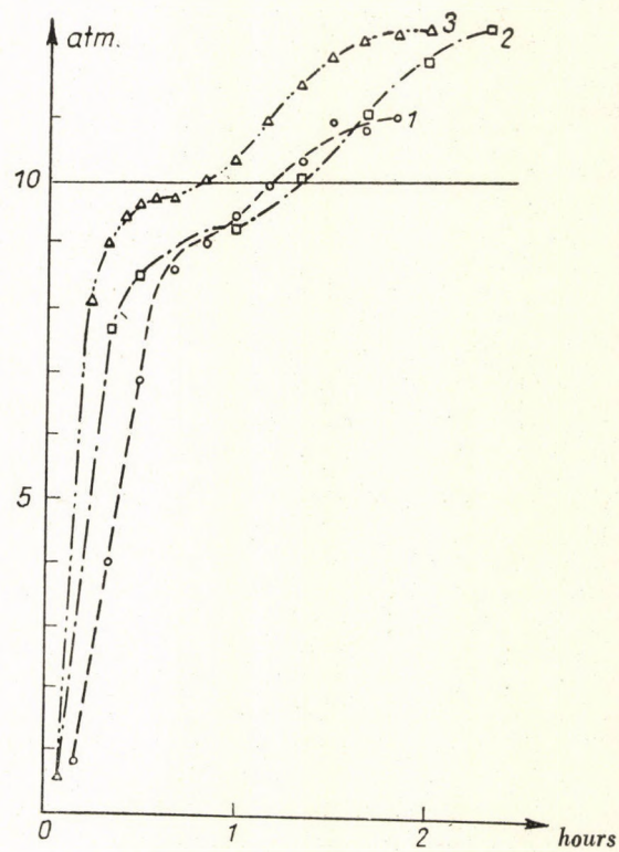
Fig. 10. Hydrogenation of benzaldehyde 1. K1, 2. K2, 3. K3
