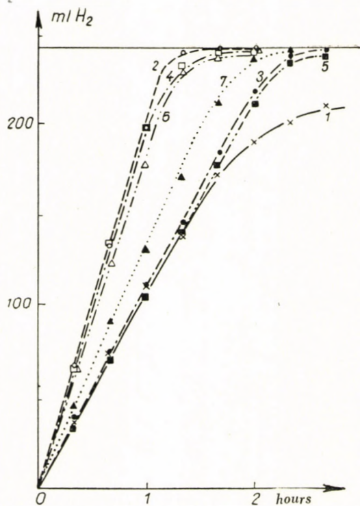
Fig. 3. Hydrogenation of eugenol
