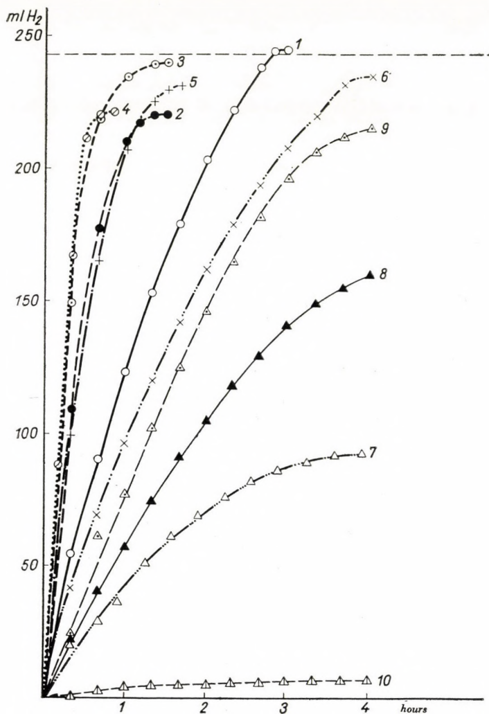
Fig. 2. Hydrogen uptake of acetone
