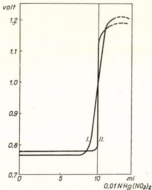
Fig. 1. Potentiometric titration of a 0,01 N solution of KCl(I), and KBr(II), respectively, with a 0,01 N solution of mercuric nitrate in the presence of iron(III) cyanide 1 ml of 1/30 M K_3[Fe(CN)_6] , 5 N H_2SO_4 ; initial volume 100 ml; saturated calomel electrode
