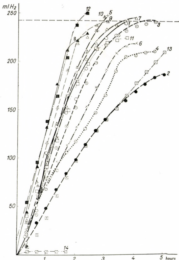
Fig. 2. Hydrogen uptake of benzophenone Legend of numbers of catalysts in Table I
