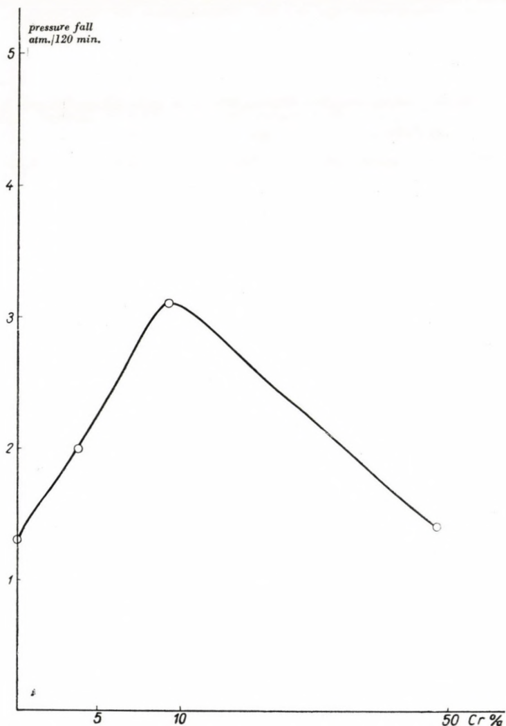
Fig. 11. Changes in activities of catalysts with veratrol, plotted against contents of cobalt
