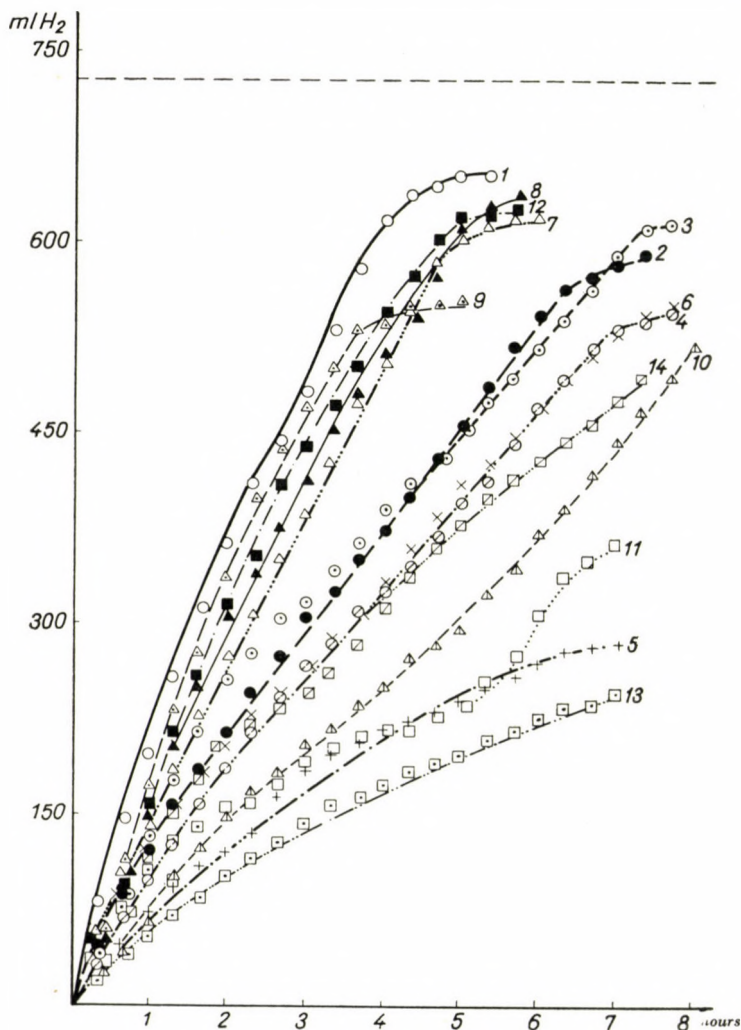
Fig. 6. Hydrogen uptake of nitrobenzene Legend of numbers of catalysts in Table I
