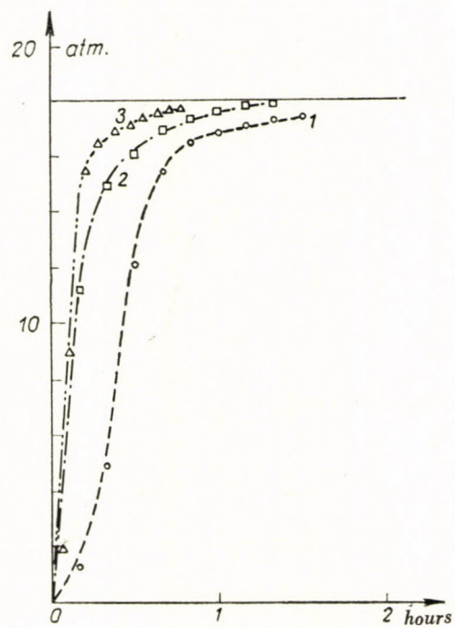
Fig. 12. Hydrogenation of benzyl cyanide 1. K1, 2. K2, 3. K3
