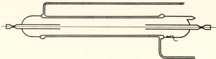
Fig. 2. Geiger—Müller-tube, type Bozóky [4], for activity measurement of flowing liquids
