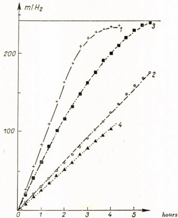
Fig. 8. Hydrogenation of benzophenone 1. Raney-Ni, 2. K4, 3. K5, 4. K6
