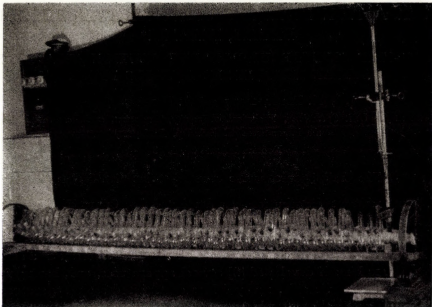
Fig. 1. Countercurrent distribution apparatus, 50 elements
