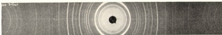
Fig. 3. Diffraction pattern of Li_2CO_3
