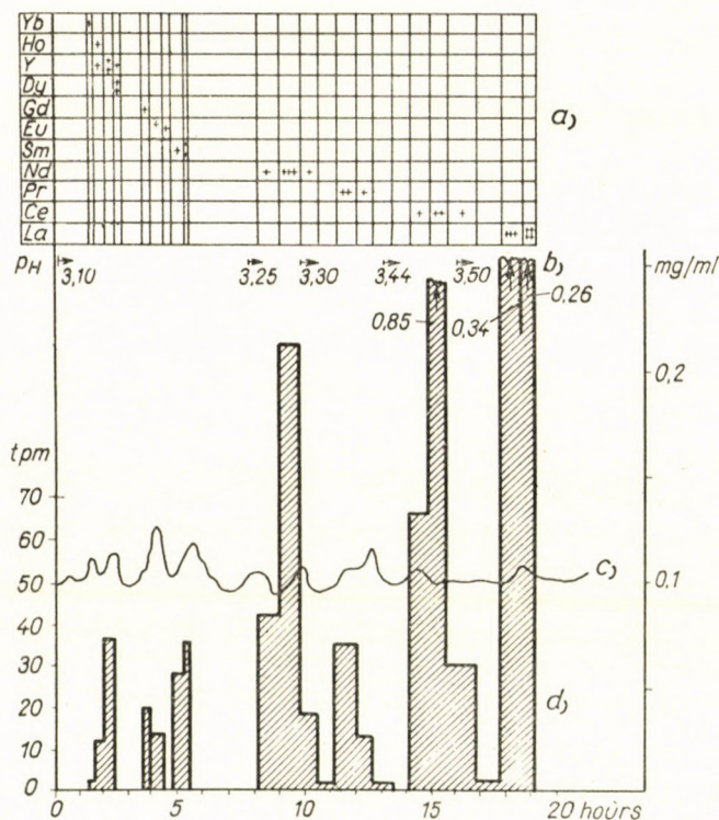
Fig. 6. Complete separation by stepwise chromatography of a sample rich in rare earth metals, recovered from Kola phosphate a) Data obtained by qualitative spectral analysis, b) original pH value of the eluent, c) activity of the effluent, d) content of rare earth metal oxides in the effluent
