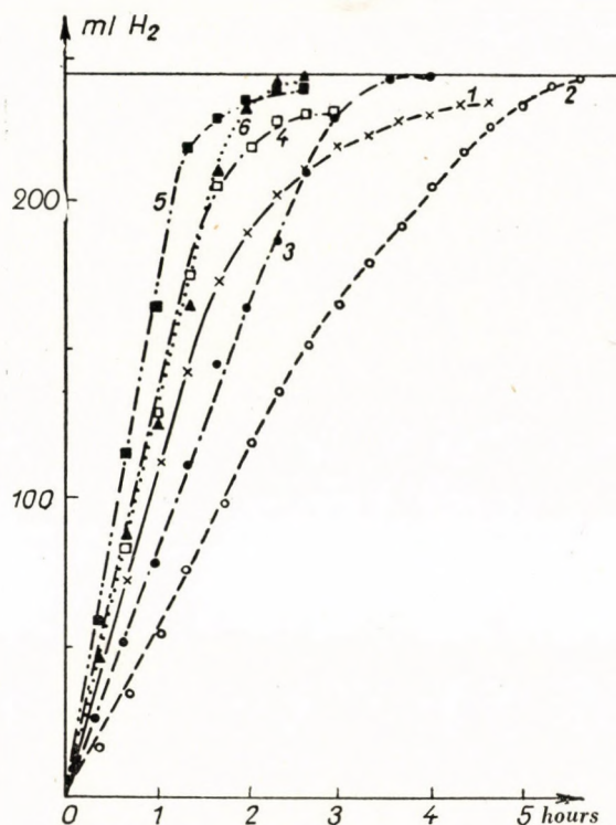
Fig. 2. Hydrogenation of eugenol
