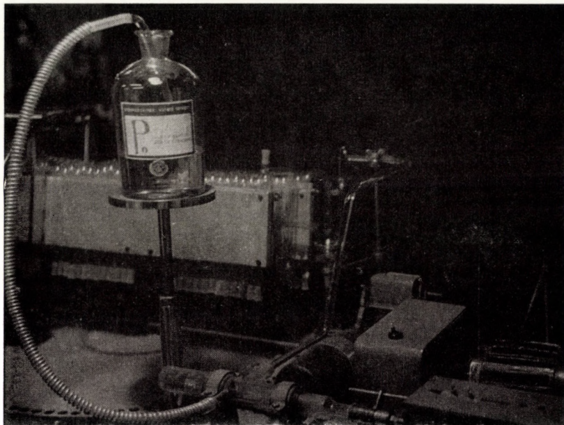
Fig. 12. Device for the automatic dosage of the solvent
