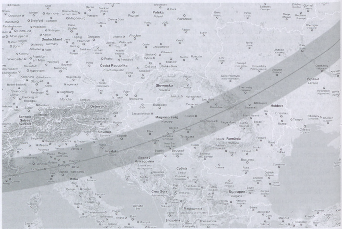
The path of annularity (99 percent) of March 23, 1270 eclipse
