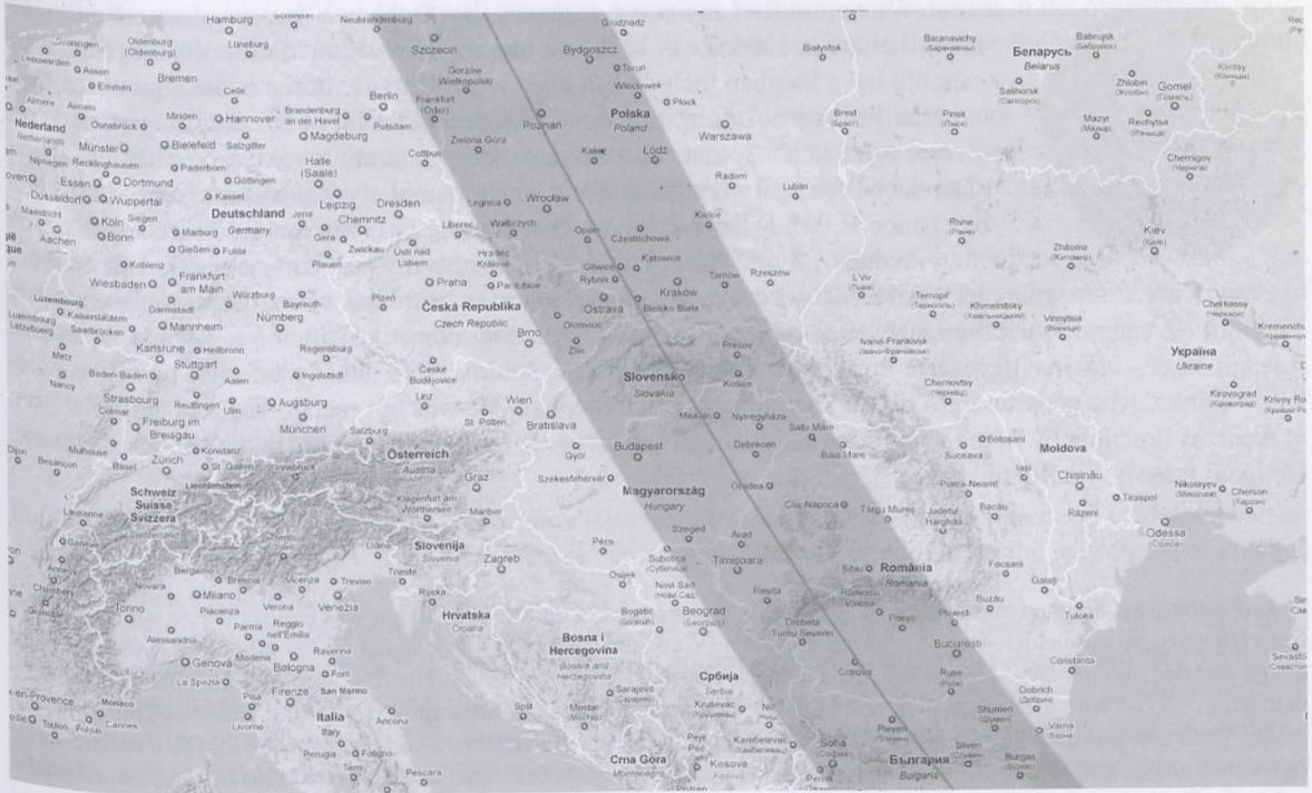
The path of annularity (97 percent) of March 5, 1263 eclipse
