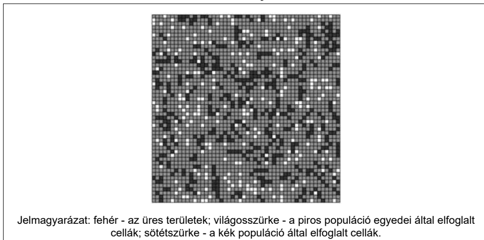
Figure 5.: No segregation pattern forms either by asymmetric population rate or by low similarity index
