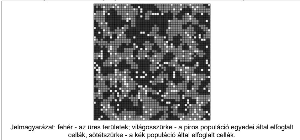
Figure 6.: Weak segregation pattern with medium similarity index
