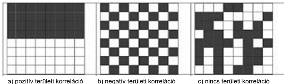
Figure 1: The cases of spatial autocorrelation
