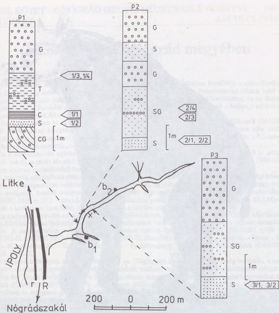
Fig 13. Sketch of the Paris Valley with the location of the investigated profiles. Legend: r: road, R: railway, b1-2: paleobotanical localities, x: locality of the Calicotherium molar , 1/1-3/2 location of the samples taken from the profiles, G: gravel, S: sand, C: clay, T: tuffitic clay, SG: sand with interbedded gravels, CG: cross bedded gravel, p1-3: profiles.
