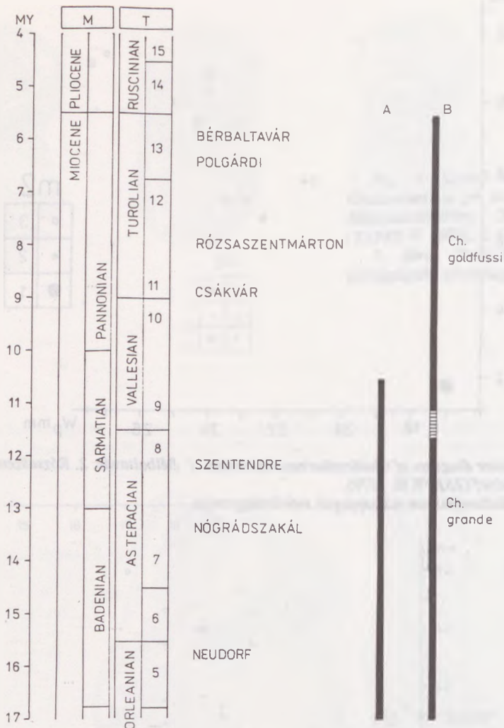
Fig. 12. The stratigraphical position of the Calicotherium localities in the Carpathian Basin.
