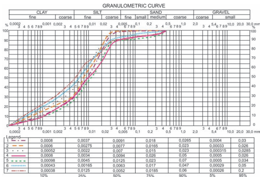
Fig. 4. Granulometric curve with triple maxima at the Szulimán section (sample N7: 4.40–4.60 m) in the paleosol superimposing grey Pannonian clay and in old loess underlying upper paleosol, interwoven with red krotovinas (Kis, É.)
