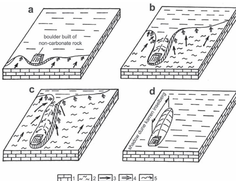
Fig. 2. The development of the 'shadow dune karren inselberg' (VERESS, M. et al. 2006). – a = the water moving to the east dissolves the surface except the part of the surface which is behind the boulder; b–c = elevation develops at the wind shadow; d = where the wind shadow surface ends the surface dissolves behind the boulder too, the elevation buds; 1 = marble; 2 = puddle; 3 = wind direction; 4 = dissolution; 5 = dissolution at sheet water
