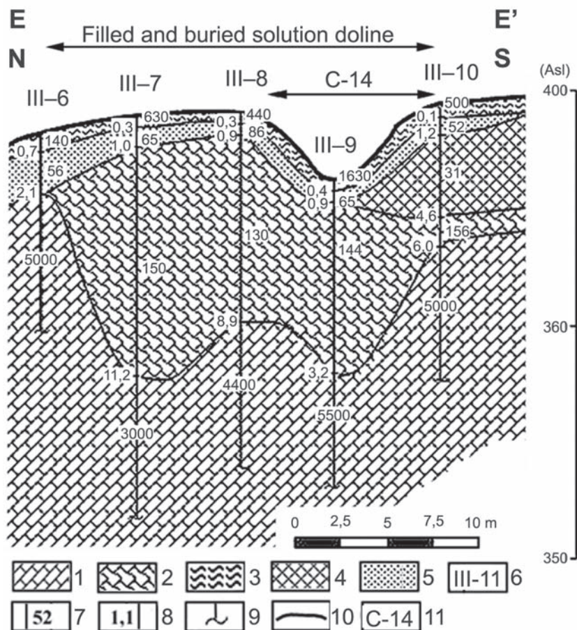
Fig. 5. Covered karst doline which developed at wedges out of permeable, filled and buried solution doline (Mecsek Mountains, from the area of Czigány land near Orfű). – 1 = limestone; 2 = limestone detritus (sand?); 3 = soil; sand; silt; 4 = clay (with limestone detritus and sand); 5 = sand, loess (with limestone detritus); 6 = number and place of VES measuring; 7 = geoelectrical resistance of the beds (Ohm); 8 = depth of the bottom of the geoelectrical beds (m); 9 = penetration of the VES measuring; 10 = border of the geoelectrical beds; 11 = mark of the covered karst form
