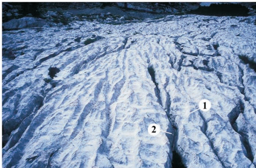
Photo 1. A bare slope with small dip angle from Totes Gebirge. – 1 = type A channel; 2 = type B channel
