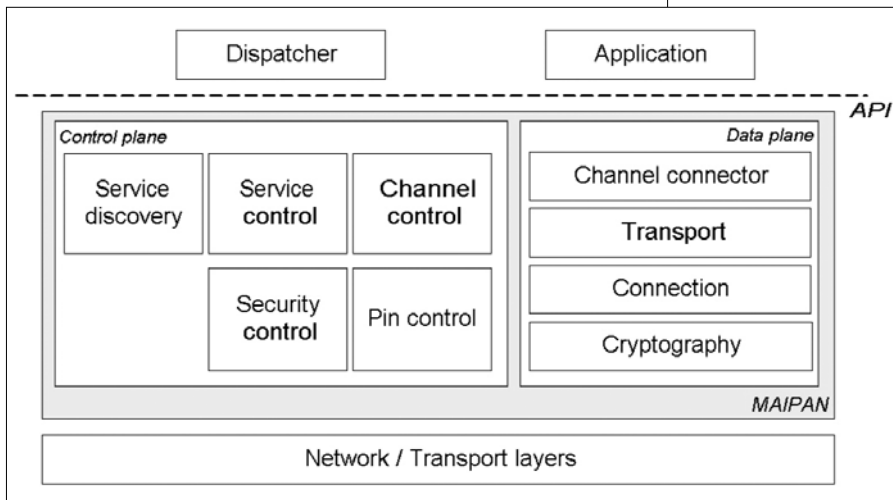
Figure 3. MAIPAN's architecture
