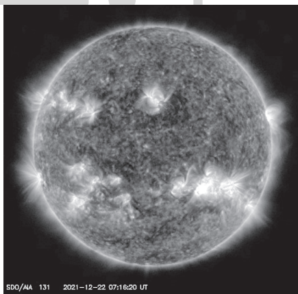
SDO/AIA 131 2021-12-22 07:16:20 UT
