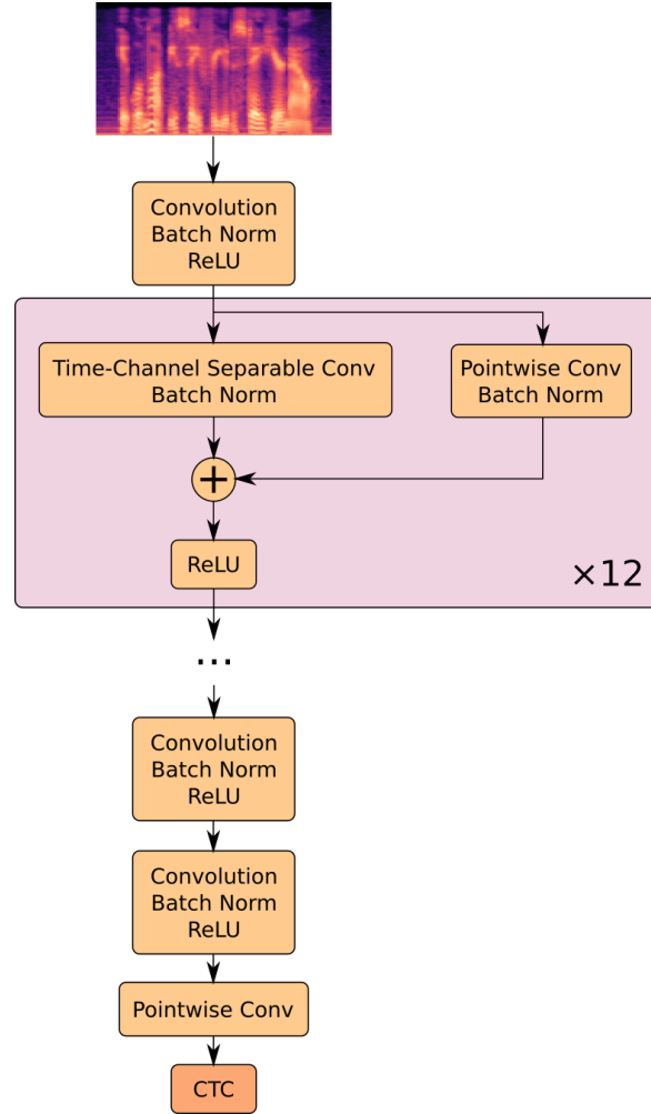
Figure 1: The QuartzNet 12 \times 1 end-to-end deep neural network architecture
