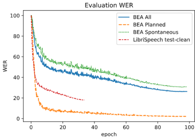
Figure 2: Evaluation WER
