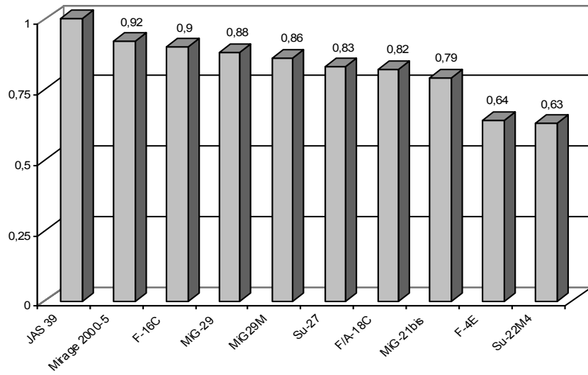
Fig.1. Manoeuvrability ranking
