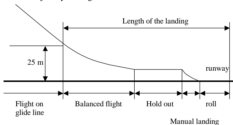
Fig. 1. Stages of the landing the UAV
