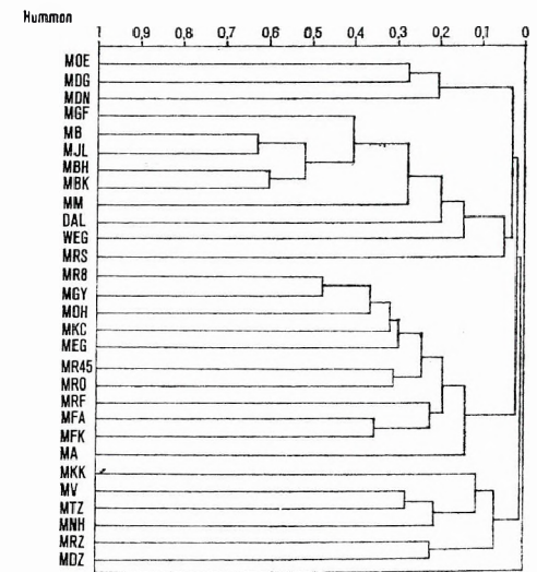
Fig. 12. Dendrograms showing similarities of species assemblages based on cluster-analysis. [Codes of assemblages (layers) are explained on pages 36—47]
