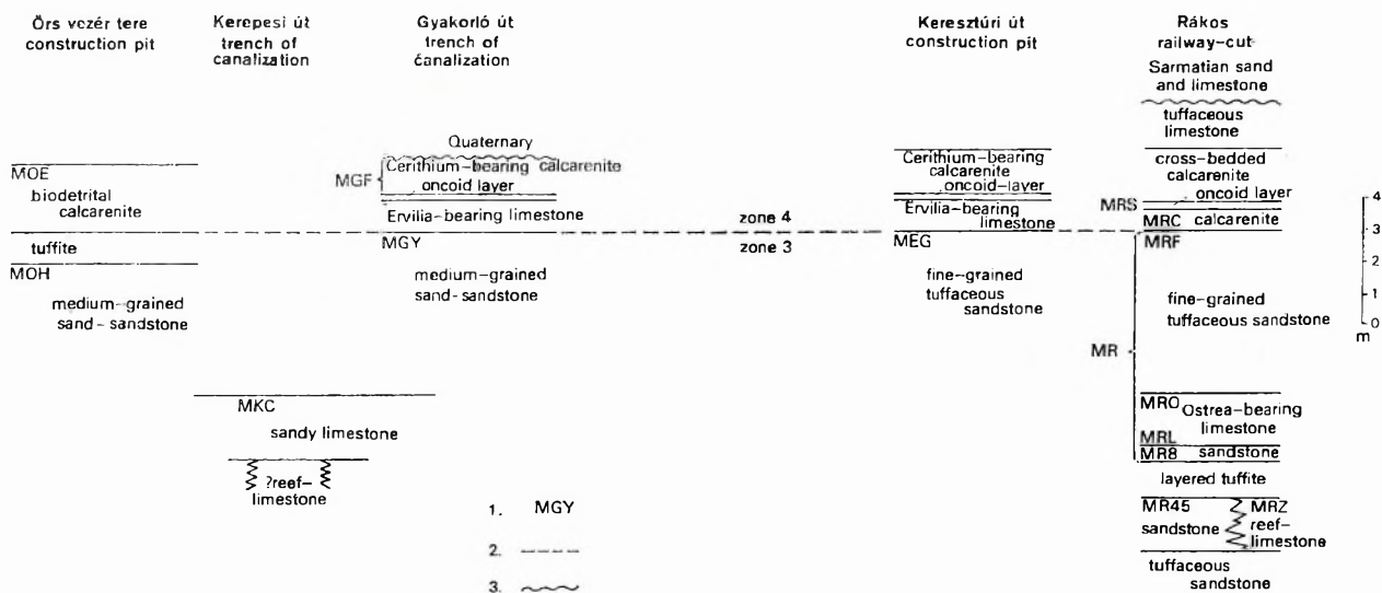
Fig. 5. Simplified section along the localities near Rákócs (horizontally not to scale) 1. Code of decapod-bearing layers, 2. boundary of biozones, 3. unconformity
