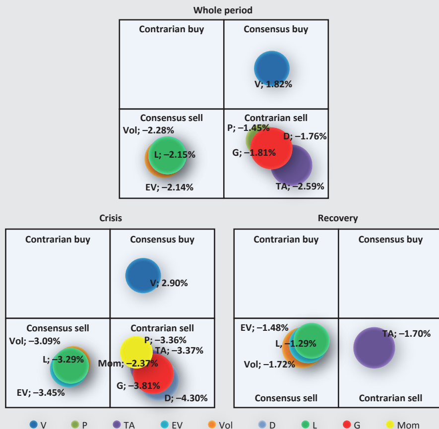
Figure 4 Significant excess returns of factor portfolios
