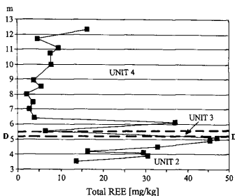
Fig. 12 Distribution of total REE content in the studied key-section, Fortuna u. 25. Unit 2: Laminated travertine, Unit 3: Palaeosol, Unit 4: Massive travertine, D—D=Discontinuity surface
