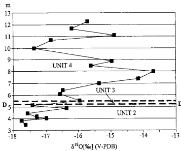
Fig. 9 \delta^{18}\text{O} (‰) composition-log of the studied key section, Fortuna u. 25. (V-PDB). Unit 2: Laminated travertine, Unit 3: Palaeosol, Unit 4: Massive travertine, D—D=Discontinuity surface
