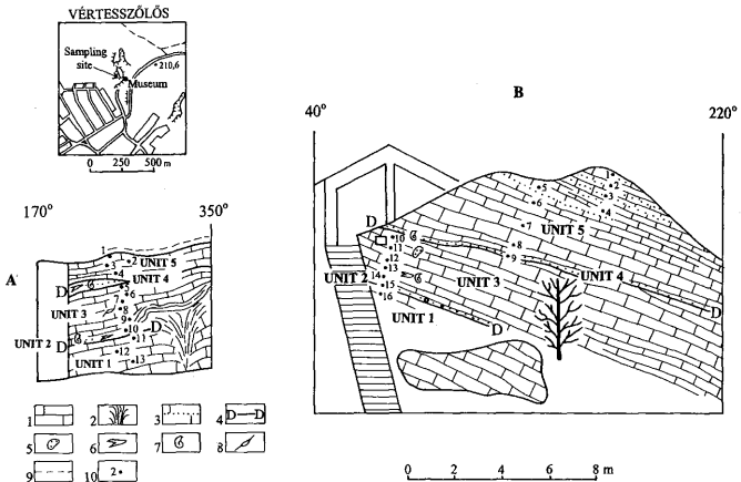
Fig. 14 Lithological profile of the travertine deposit at Vértesszőlös (A = profile of the "Lorelei stone" B = profile of the step) (KORPÁS 2003b). 1 Travertine, 2 Spring throat with laminated travertine, 3 Fine sand, 4 Discontinuity surface, 5 Place of occurrence of the os occiput, 6 Other Os remnant, 7 Gastropod remnants, 8 Leaf print, 9 "Culture layer No 3", 10 Place of sample
