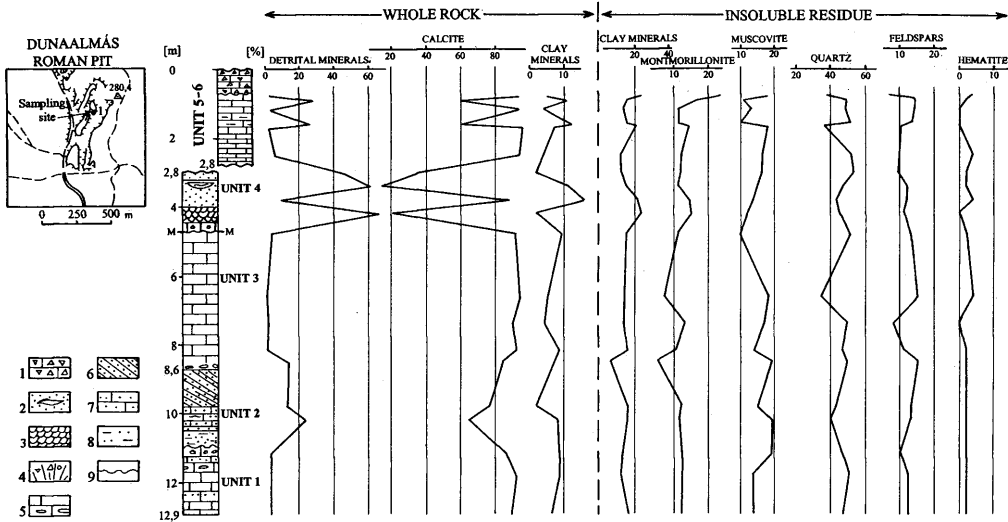
Fig. 8 Lithological column of the profile of Dunaalmás-1 (KORPÁS 2003b), and its mineralogical composition. 1. Travertine breccia, 2 Sand with clay lenses, 3 Palaeosol A level, 4 Palaeosol rooted B level, 5 Well-bedded travertine with sedge and cane remnants, 6 Cross-stratified sand, 7 Oolitic travertine, 8 Clayey sand, 9 Discontinuity surface
