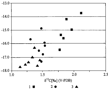
Fig. 10 \delta^{13}\text{C} (‰) and \delta^{18}\text{O} (‰) diagram of different types of travertine. 1. Massive travertine of Unit 4, 2. Laminated travertine of Unit 4, 3. Laminated travertine of Unit 2
