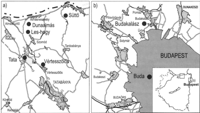
Fig. 1 Quaternary travertines in north-eastern Hungary (KORPÁS 2003b)
