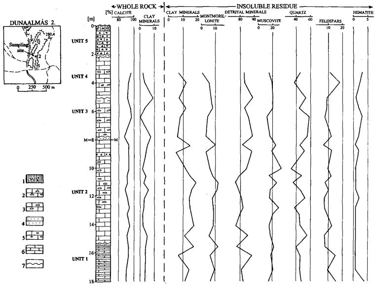
Fig. 9 Lithological column of the profile Dunaalmás-2 (KORPÁS 2003b), and its mineralogical composition. 1 Earthy travertine breccia, 2 Travertine breccia, 3 Well-bedded travertine with sedge and cane remnants, 4 Sand, 5 Pebbly sand, 6 Laminated travertine, 7 Discontinuity surface
