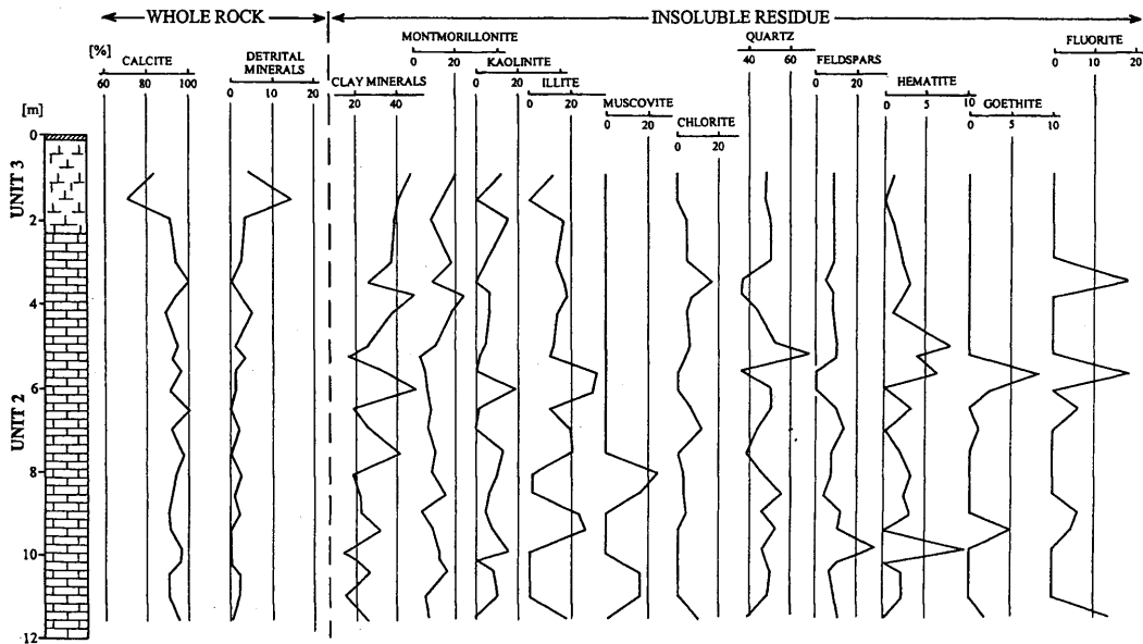
Fig. 3 Mineralogical composition of the travertine from Budakalász (for legend see Fig. 2)
