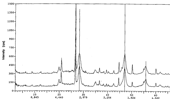
Fig. 16 XRD patterns of samples containing fluorite (Budakalász 3.45 m, Süttö: Diós-valley 13.10 m)
