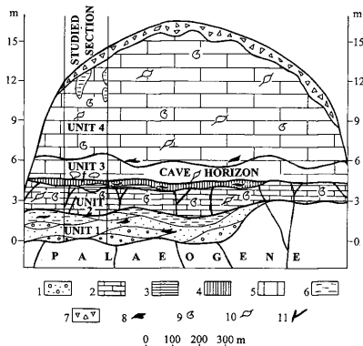
Fig. 3 Stratigraphic chart of the Vár-hegy travertine. 1 Basal clastics, 2 Laminated travertine, 3 Laminated limy mud cavity fill, 4 Palaeosol horizon, 5 Massive, crystalline travertine, 6 Red clay fissure fill, 7 Loose cover sediments, 8 Vertebrates, 9 Gastropods, 10 Plants, 11 Open fissures
