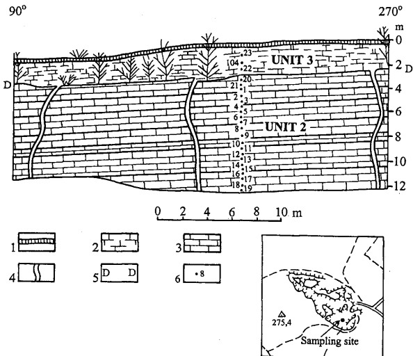
Fig. 2 Lithological profile of the travertine at Budakalász (KORPÁS 2003b). 1 Soil, 2 Brecciated, autoclastic travertine, 3 Laminated travertine, 4 loess-like chalk sediments in fissure, 5 Discontinuity surface, 6 Place of sample (without 1st unit)
