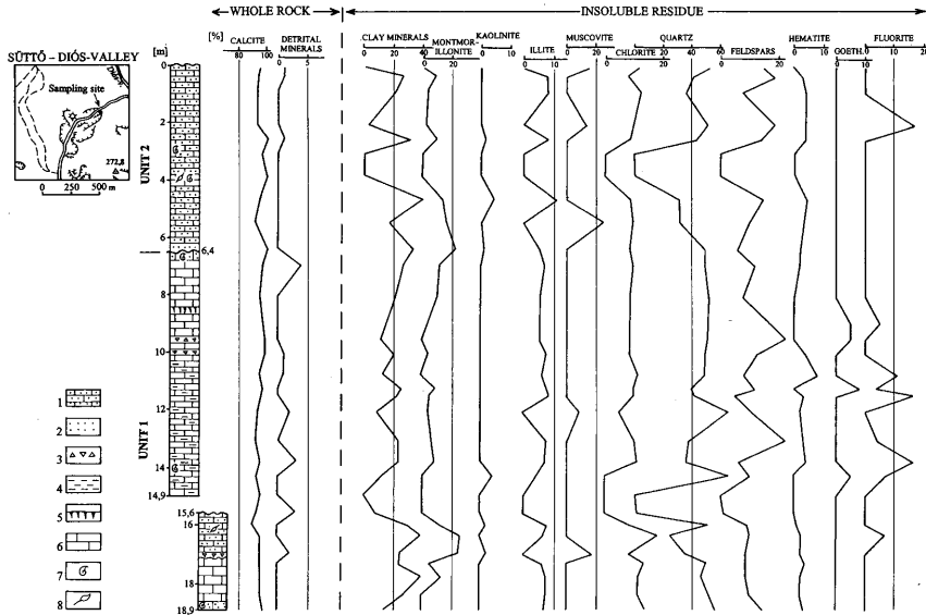
Fig. 4 Lithological profile of the travertine deposit at Diós valley, Süttő (KORPÁS 2003b), and its mineralogical composition. 1 Oolithic travertine, 2 Micaceous (Muscovitic) sand, 3 Fragmented travertine, 4 Bird's eye structures, 5 Rooted horizon, 6 Well-bedded travertine, 7 Gastropod remnants, 8. Plant remnants
