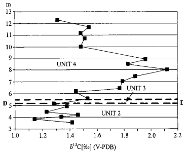
Fig. 8 \delta^{13}\text{C} (‰) composition-log of the studied key section, Fortuna u. 25. (V-PDB). Unit 2: Laminated travertine, Unit 3: Palaeosol, Unit 4: Massive travertine, D—D=Discontinuity surface
