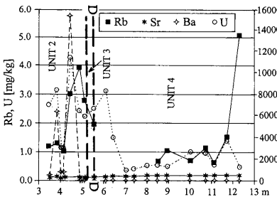
Fig. 14 Distribution of Rb, Sr, Ba and U contents in the studied key-section, Fortuna u. 25. Unit 2: Laminated travertine, Unit 3: Palaeosol, Unit 4: Massive travertine, D—D=Discontinuity surface
