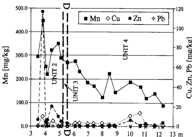
Fig. 15 Distribution of Mn, Cu, Zn and Pb contents in the studied key-section, Fortuna u. 25. Unit 2: Laminated travertine, Unit 3: Palaeosol, Unit 4: Massive travertine, D—D=Discontinuity surface
