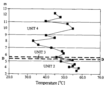
Fig. 11 Log of calculated precipitation-temperatures of the studied key-section, Fortuna u. 25. Unit 2: Laminated travertine, Unit 3: Palaeosol, Unit 4: Massive travertine, D—D=Discontinuity surface
