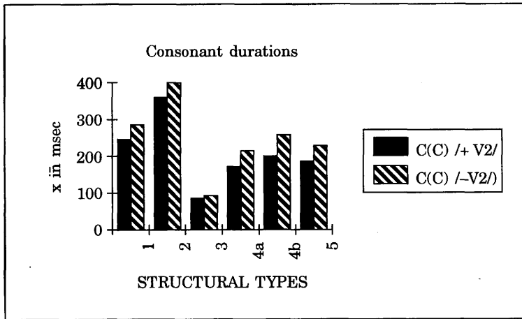
Figure 2. Consonants durations
