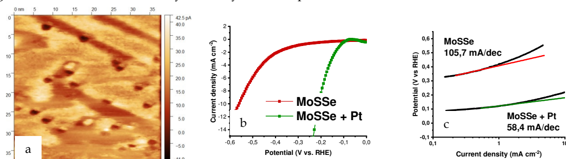
Figure 1: STS map showing S and Se rich regions in a MoS 2 Se layer (a). Linear sweep voltammogram curves (b) and corresponding Tafel plots (c) for MoS 2 Se and MoS 2 Se+Pt samples. In (b) the potential was measured versus a reversible hydrogen electrode - (RHE) reference electrode.
