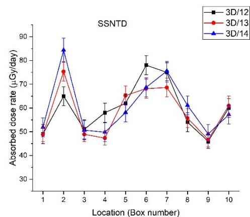
Figure 2: Absorbed dose rates measured by SSNTDs
