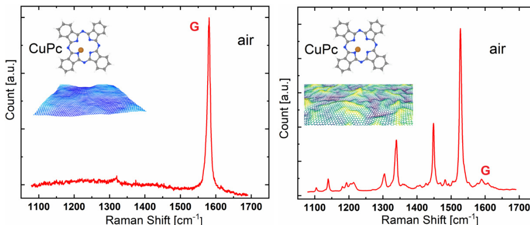
Figure 2: (right) Huge Raman enhancement on nanocorrugated graphene sheets. Detection of CuPc molecules from “clean” air by nanocorrugated graphene sheets. (left) The Raman spectrum of quasi-flat graphene subjected to the same conditions is shown for reference.
