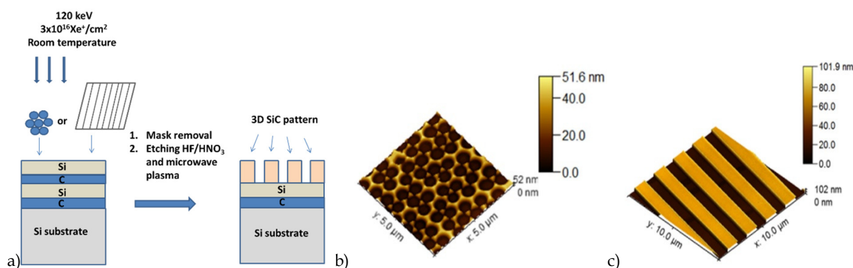
Figure 1: a) Process of producing 3D structures b) AFM image of the LB-masked sample after mask removal and one step HF/HNO 3 etching and one step oxidation. c) AFM image the grid-masked sample after mask removal and HF/HNO 3 etching, oxidation and additional HF/HNO 3 etching
