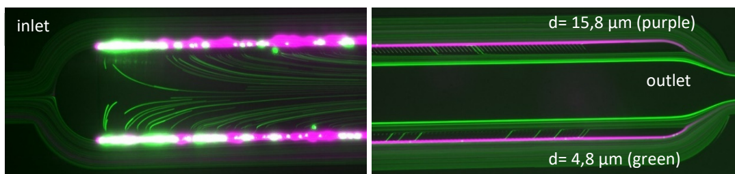
Figure 4: Size dependent filtration of different fluorescent beads in cross-flow type microfluidic separation system (at 3µL/s flow rate)
