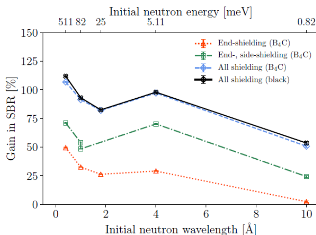
Figure 1: Simulated Signal-to-Background Ratio with combined shielding with boron-carbide compared to black material, normalised to the unshielded reference detector.
