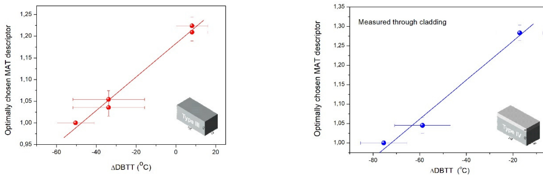
Figure 3: Correlation between normalized MAT parameters and transition temperature, measured directly on base material (left) and on cladding (right)
