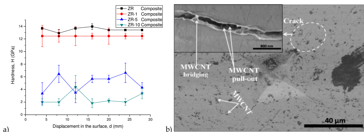
Figure 1: Mechanical properties of 8YSZ/MWCNTs composites. a) hardness measurements, b) crack propagation in composite with 1 wt% MWCNTs
