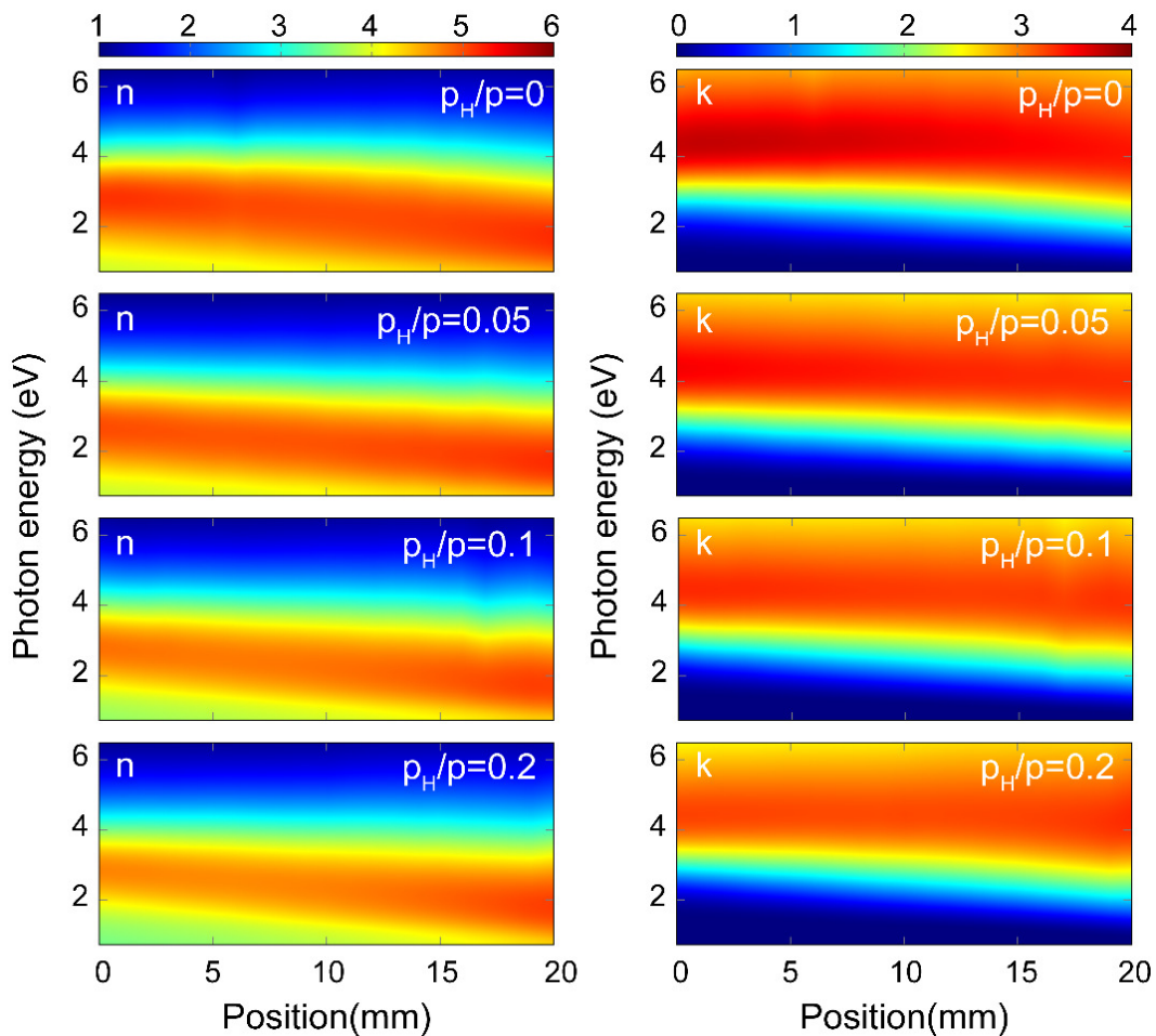
Figure 2: Real and imaginary parts of the complex refractive indices of a\text{-Si}_{1-x}\text{Ge}_x\text{:H} thin films (left and right column, respectively) with different partial pressures of H ( p_{\text{H}}/p = 0; 0.05, 0.1 and 0.2 ) as a function of both the position along the 20 mm long gradient section (composition) and photon energy. According to the RBS plots, the position at 0 mm corresponds to the Si-side of the sample.
