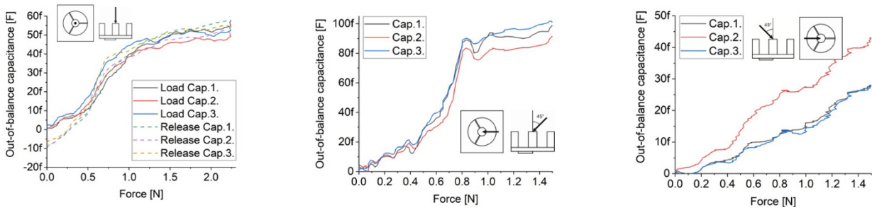
Figure 3: Responses of the three elements for the three characteristic directions as indicated with the insets.
