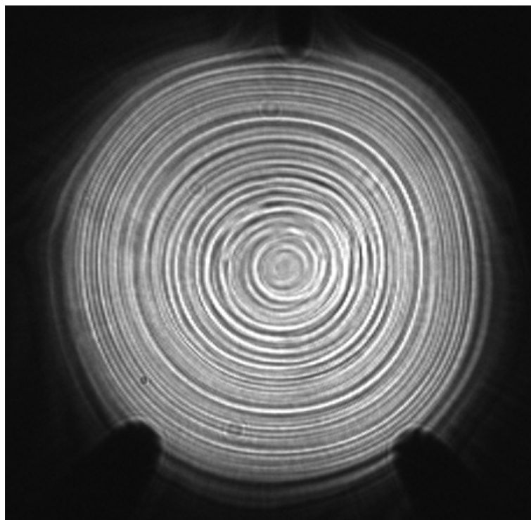
Figure1: Typical Makyoh-topography image of a swirl defect in a p -type Si wafer
