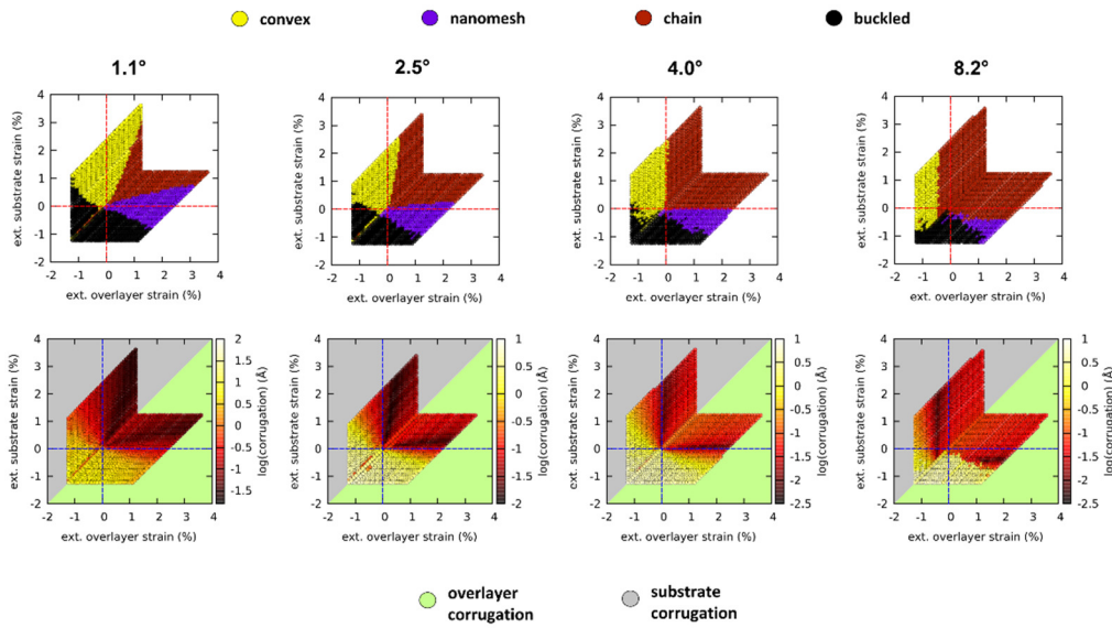
Figure 3: Top row: Moiré-phases of the twisted trilayer graphene system for different twist angles in the space of externally applied homogeneous strains (phase-maps). The corresponding Moiré-phases are indicated with different colours (yellow - convex, purple - nanomesh, red - chain). Bottom row: The same phase-maps but coloured by the corrugation of the relaxed Moiré-superlattices. The dark areas show the ultra-flat states around the phase boundaries.
