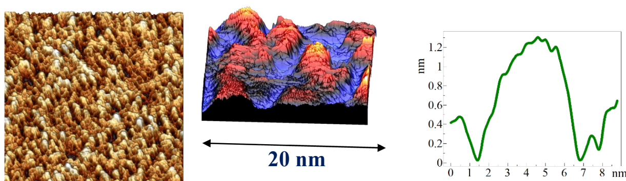
Figure 1: The structure of nanobuckled graphene sheets. STM images of graphene sheets prepared by cyclic thermal annealing displaying a particularly strong nanoscale corrugation, with lateral size below 10 nm, and nanometer height. Line cut displaying a typical graphene nanocorrugation geometry with an aspect ratio of h_{\text{max}}/R \sim 0.5 .
