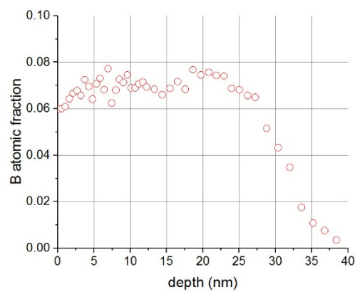
Figure 2: AES depth profile from native surface of the implanted layer
