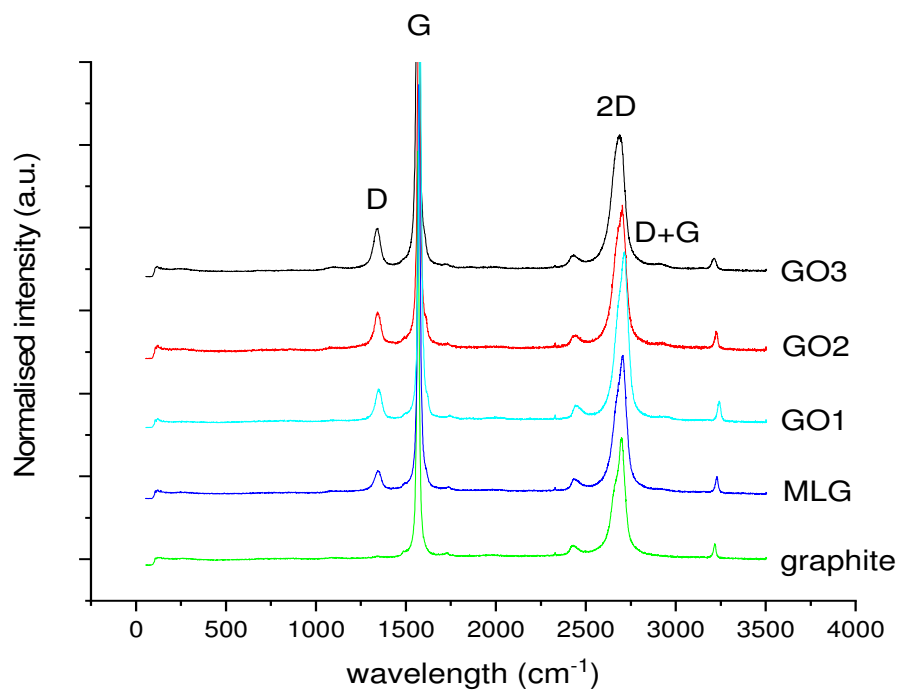
Figure 2: Raman spectra of graphite, MLG and different graphene oxide samples
