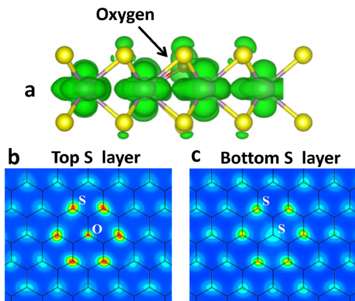
Figure 3: Electronic density of states redistribution near the O substitution site in MoS 2 single layer. In-plane view of the S layers highlighting increased electron density on the nearest neighbor S atoms.
