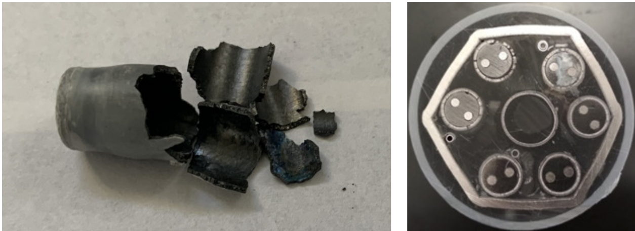
Figure 1: Broken cladding pieces from the top of the bundle (left) and cross section of the bundle at 550 mm elevation
