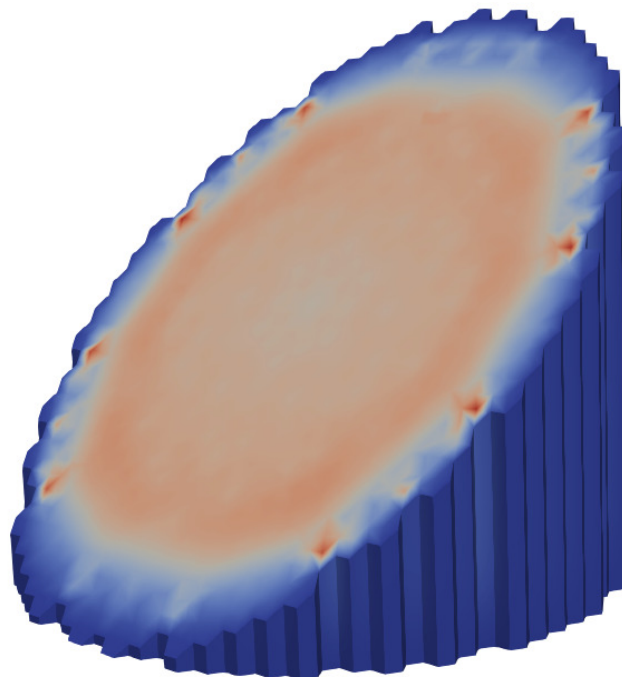
Figure 1: Distribution of thermic neutrons in the reactor core during the measurement made at the end of the fuel cycle
