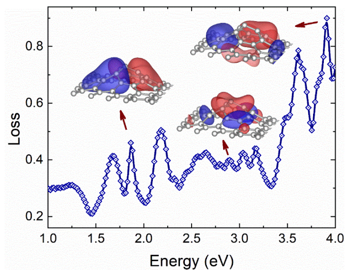
Figure 3: Plasmonic excitations in nanocorrugated graphene. Calculated EELS spectrum of a model graphene nanocorrugation, revealing several loss peaks in the visible range. The insets display the charge distributions of optical excitations corresponding to different loss peaks.
