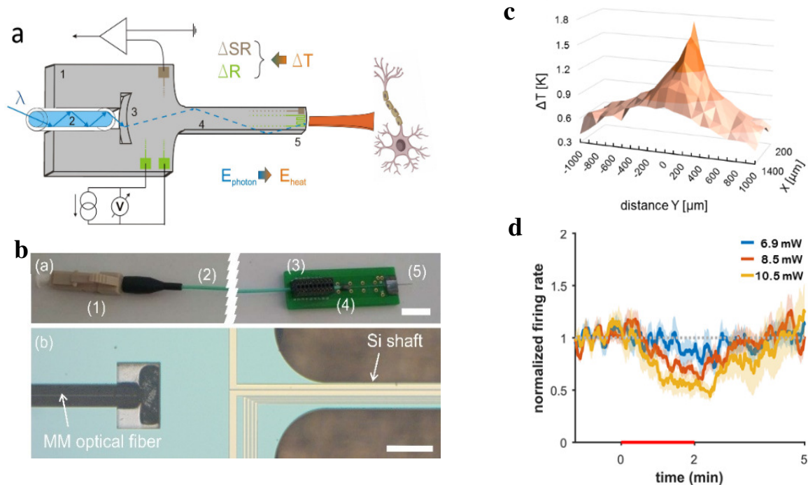
Figure 3: (a) Operation of the multifunctional probe chip designed to deliver infrared light into the neural tissue and monitor electrophysiology concurrently. (b) Photo on the ready-to-use device (top) and microscopy image of coupling region of the chip (bottom). Denoted parts: (1) optical connector, (2) optical fiber, (3) electrical connector, (4) PCB, (5) silicon chip. (c) Measured spatial distribution of temperature change evoked by the absorbed IR light around the probe shaft. (d) Representative cellular response in the cortex to IR stimulation at various input optical power.
