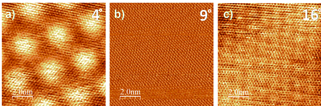
Figure 3: Topographic scanning tunnelling microscope images of graphene layers deposited on top of a graphite substrate for various relative rotation angles. The STM image in panel (b) reveals an ultra-flat state, much smoother than observed even for high rotation angles (c). The experimental conditions for image acquisition ( I_{tunnel} = 1nA , U_{bias} = 200mV ), data processing, and graphic display parameters are the same for all panels.
