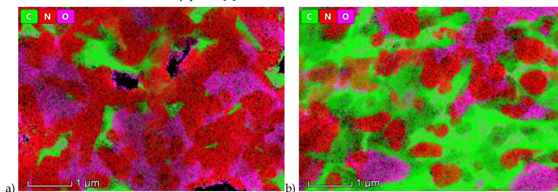
Figure 2: Elemental maps of graphene reinforced \text{Si}_3\text{N}_4 based composites: a) 5 wt% graphene, b) 30 wt% graphene
