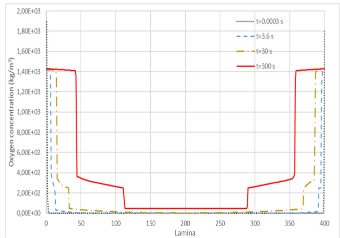
Figure 2: Calculated time evolution of oxygen concentration in the cladding
