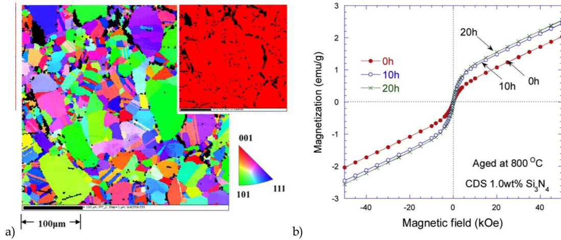
Figure 2: a) EBSD inverse pole figure (IPF) map of CDS samples with 1.0 wt% Si 3 N 4 for ageing time of 20 h, showing crystal orientation along the normal direction of sample surface. The insets show phase colour map. The crystal structure of Si 3 N 4 was not considered in this analysis, b) Magnetization curves for 1.0 wt.% Si 3 N 4 CDS samples aged at 800 °C.
