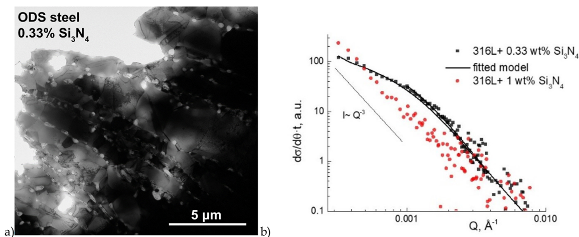
Figure 1: Si 3 N 4 ceramic dispersed strengthened steel. a) structure, b) SANS measurements
