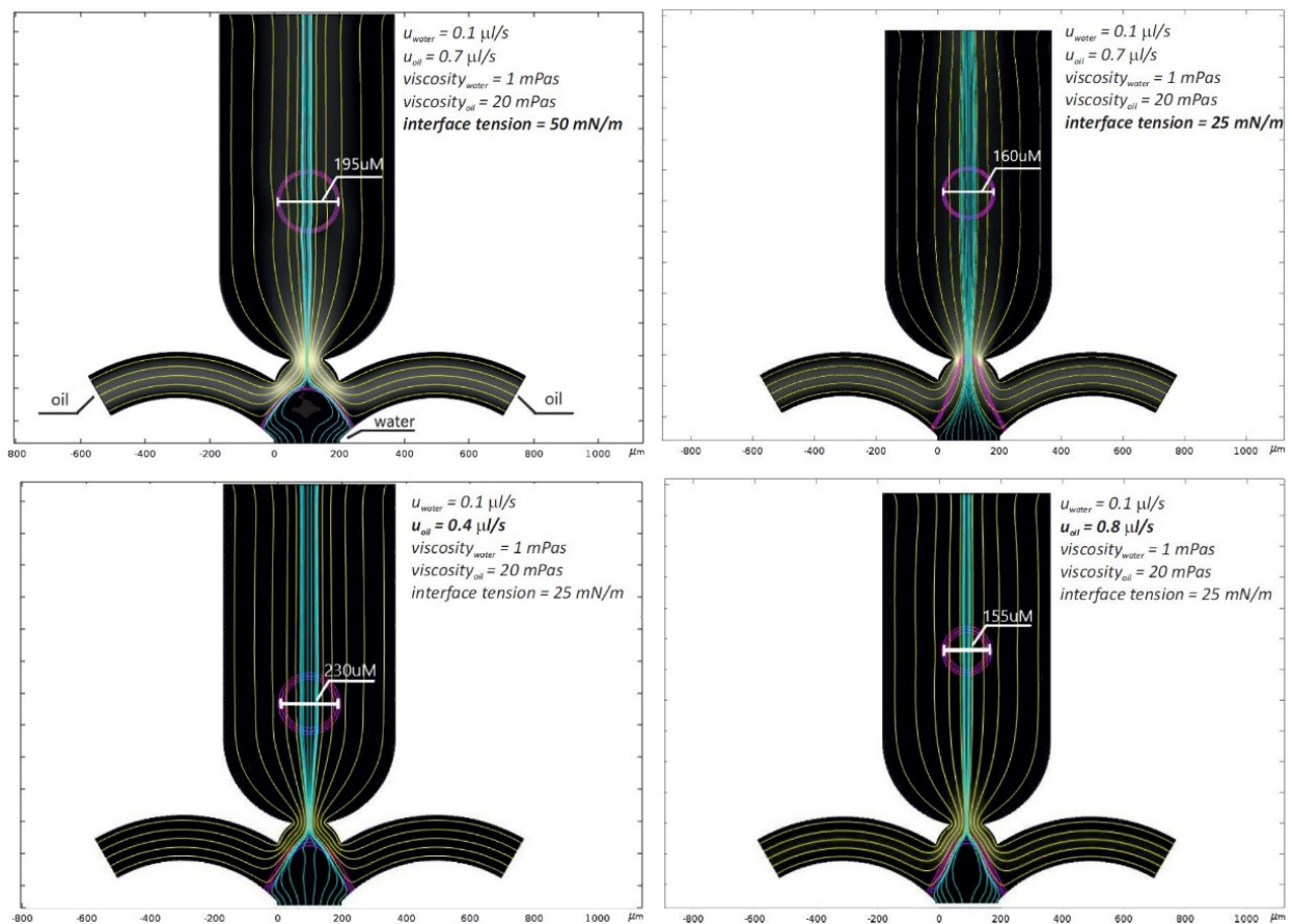
Figure 2: Influence of the interface tension and flow rate ratios on the droplet formation process (droplet size) – FEM simulation
