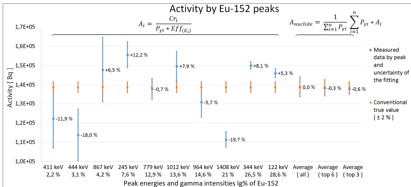
Figure 1: Activities measured/calculated from one or several peaks on the same spectrum with a RID
