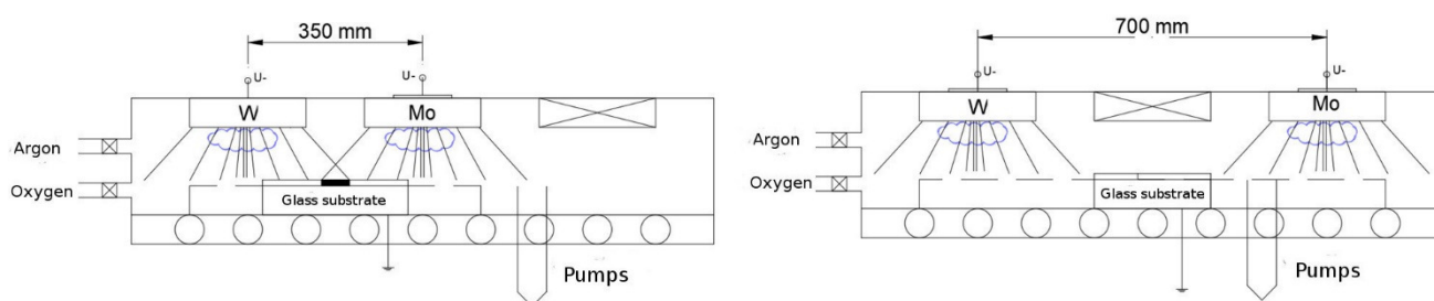
Figure 1: Two arrangements of the targets: a) the two targets in closer position (35 cm from each other) b) the two targets in distant position (70 cm from each other).
