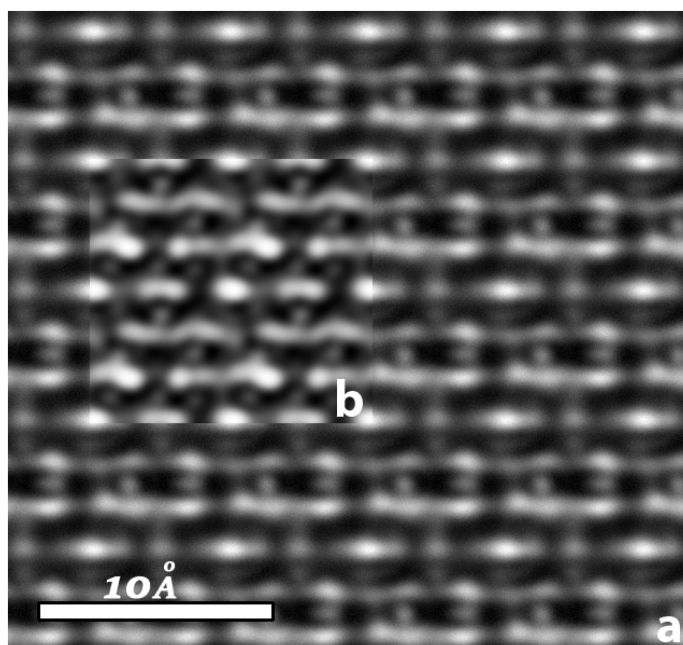
Figure 1: a) Fourier-filtered experimental HRTEM image of S_6 and b) its built structure's simulated HRTEM image
