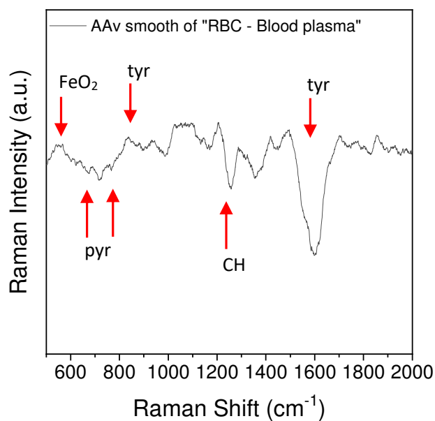
Figure 2: Differential SERS spectrum of the RBC and plasma, obtained by subtraction of normalized plasma SERS spectrum from RBC SERS spectrum. Peaks at: 570\text{cm}^{-1} ( \text{FeO}_2 ), 670\text{cm}^{-1} and 750\text{cm}^{-1} (pyrrole - pyr), 820\text{cm}^{-1} and 1550\text{cm}^{-1} (tyrosine - tyr and phenylalanine), 1227\text{cm}^{-1} (CH group of hemoglobin).
