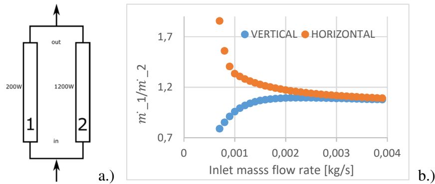
Figure 1: a.) The physical model. b.) The mass flow rate ratio between the two channels in the function of the inlet mass flow rate.
