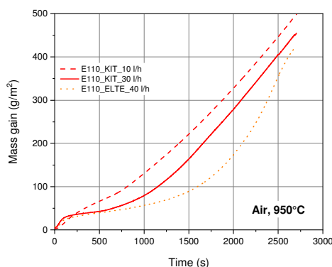
Figure 1: Comparison of mass gain of E110 tube segments oxidised at 950 °C at different air flow rates in TG
