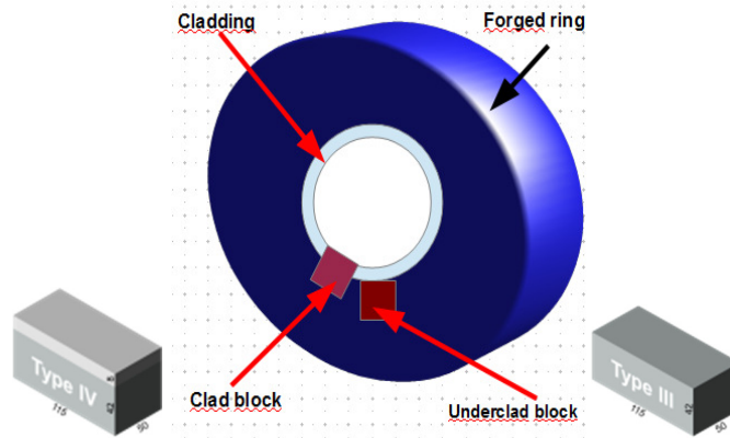
Figure 2: Cutting of clad and unclad blocks from forged ring
