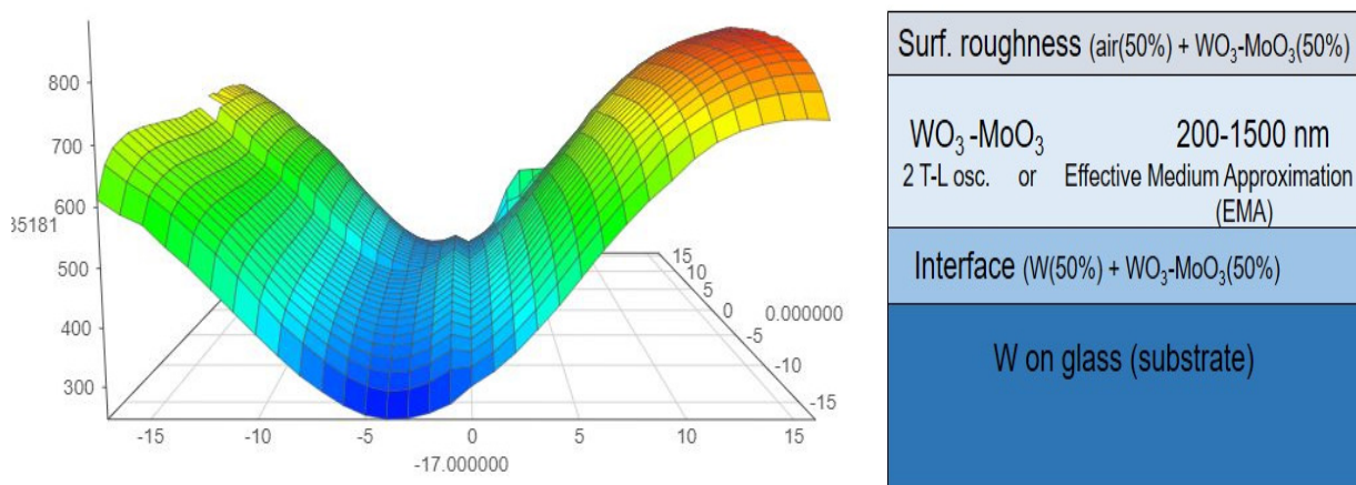
Figure 2: Thickness-map based on Tauc-Lorentz oscillator model
