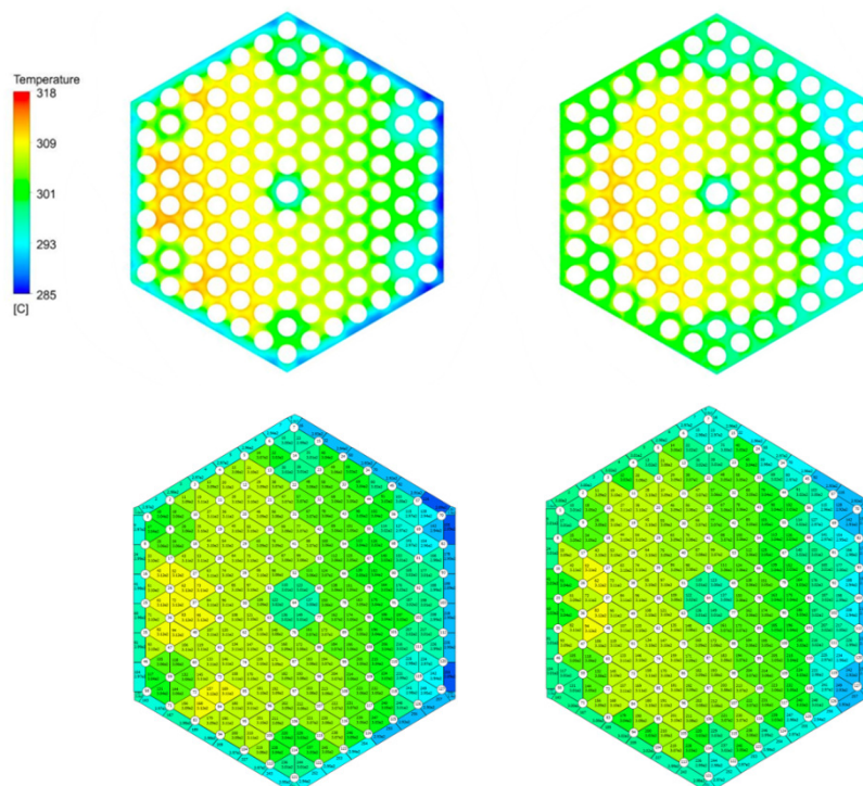
Figure 1: Distributions of outlet water temperature (top: CFD calculation; bottom: SURET calculation; left: without mixing vane; right: with mixing vane)
