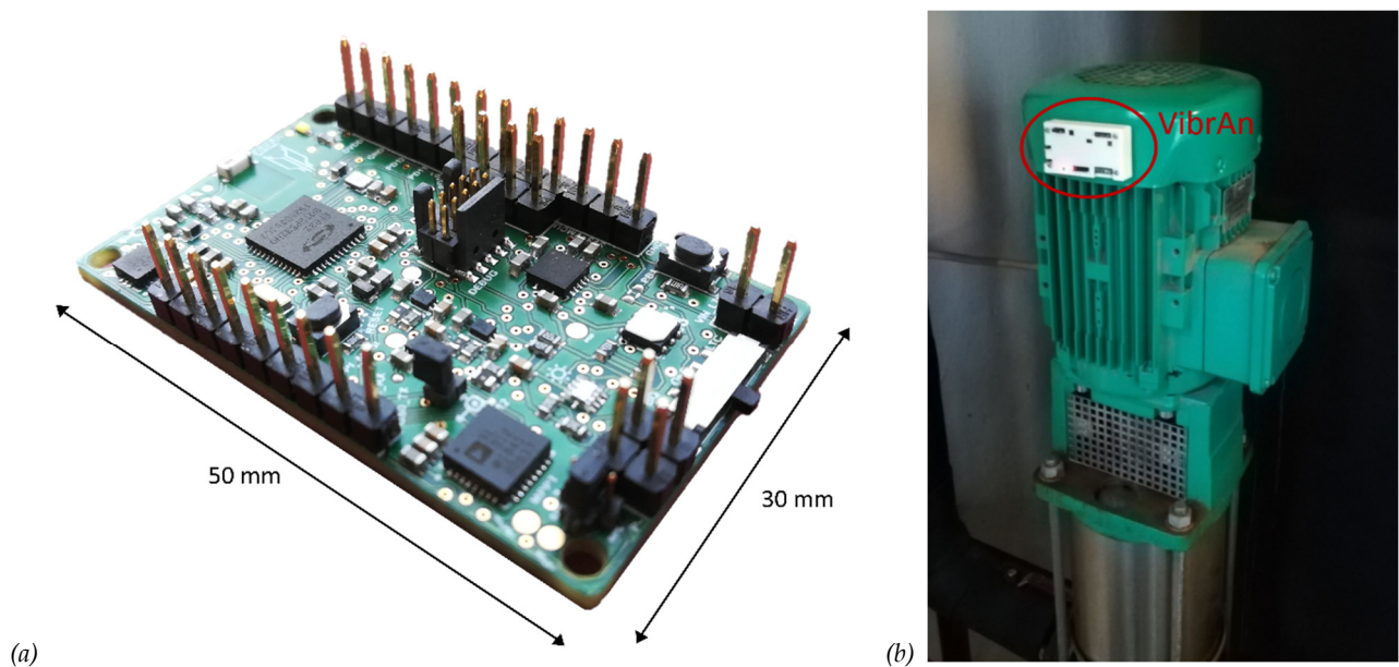
Figure 1: (a) The vibration analyser circuit board and (b) measurement setup in the engine room of building 29/B attached to an air-ventilation pump
