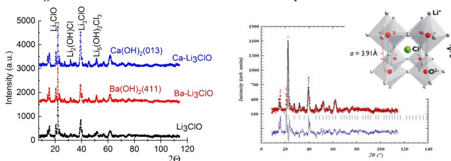
Figure 1: Neutron diffraction results for \text{Li}_3\text{ClO} -based samples
