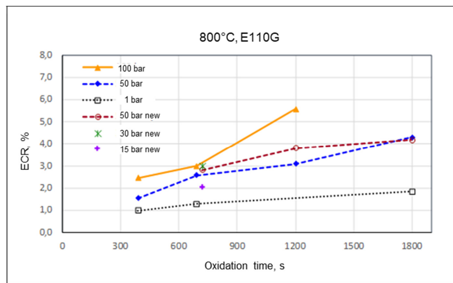
Figure 1: Influence of pressure on the oxidation kinetics of E110G alloy in steam at 800 °C
