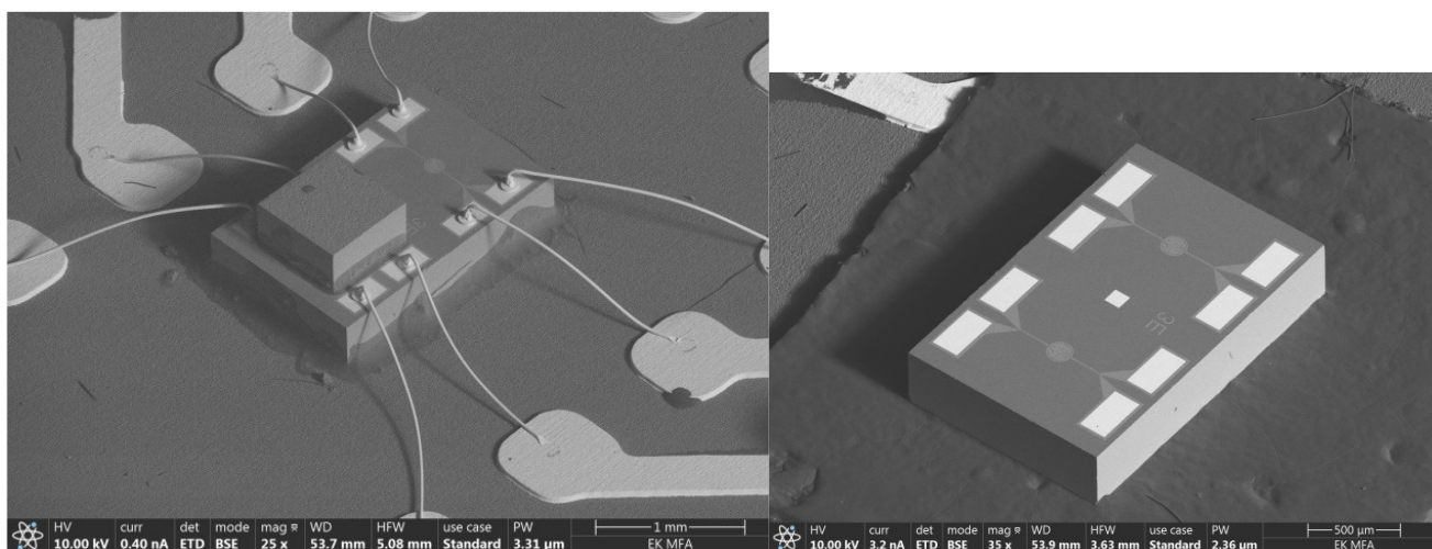
Figure 1: Construction of the heat conductivity sensor. The two identical micro-hotplates (left) and one of the hotplates are vacuum-sealed(right). The chip is mounted on a small PCB for testing.
