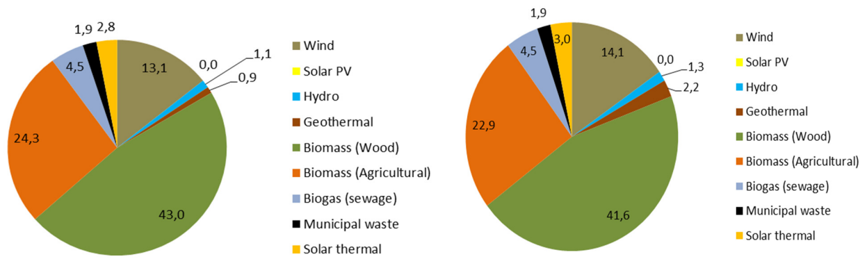
Figure 1: Optimal national portfolio of renewable energy sources with respect to economic impacts only (left) and additionally to human health, environmental and climate impacts (right).
