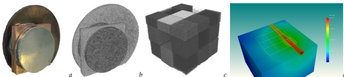
Figure 2: Photo (a) and neutron tomogram (b) of pure copper and tin, as well as a bronze reference material. Thermal-neutron tomogram of a multi-material magic cube (c), and the related MCNP6 Monte Carlo calculation (d)
