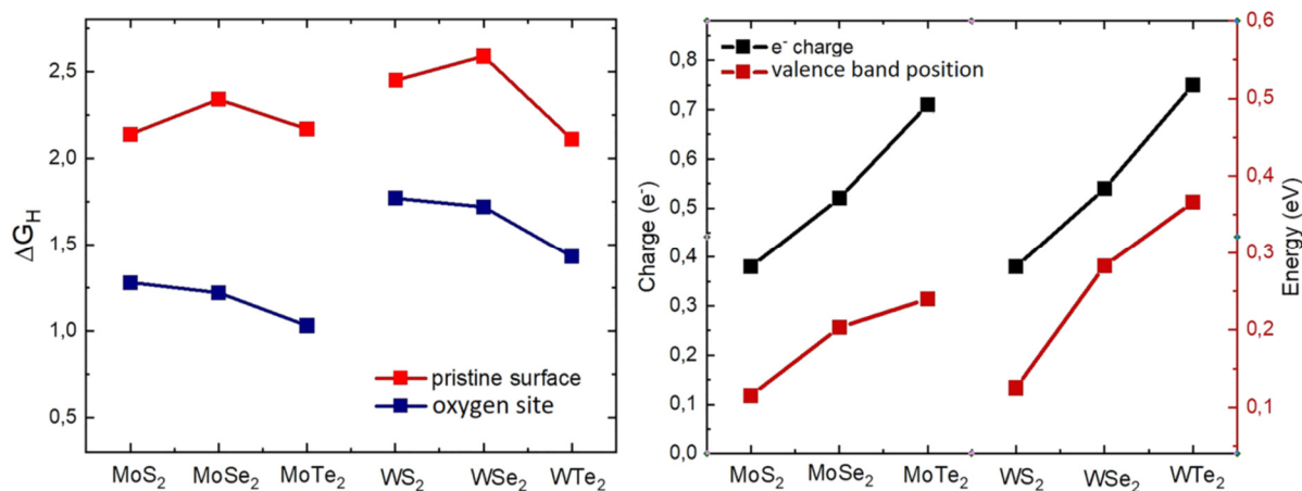
Figure 2: (left) Hydrogen adsorption Gibbs free energy on the basal plane chalcogen sites (red) and O substitution sites (blue). (right) Electron charge surplus on the O sites relative to pristine chalcogen atom sites and the position of the valence band at the \Gamma point of the Brillouin zone relative to Fermi level for various 2D TMC crystals with O substitution sites.
