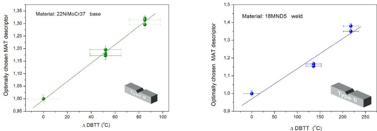
Figure 1: (left) Optimally chosen normalized MAT descriptor as a function of the transition temperature shift for a 22NiMoCr37 type base material and (right) for a 18MND5 type weld material, measured on Charpy samples.
