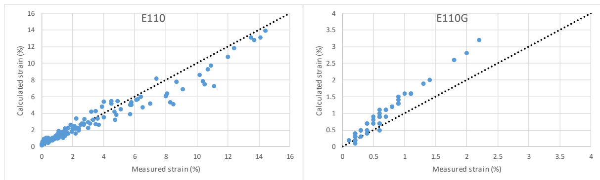
Figure 1: Calculated vs. measured tangential strains for experiments performed in the reactor BOR-60, using the flux to radiation damage conversion that gave the best results
