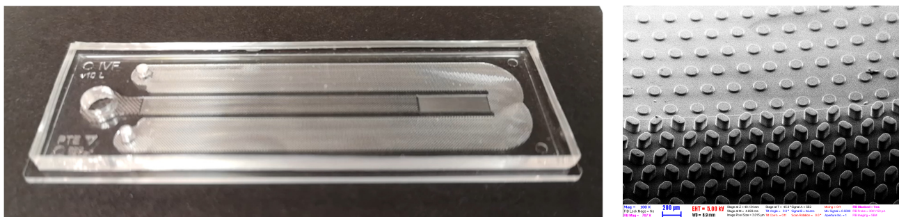
Figure 1: The autonomous microfluidic cartridge proposed for transport culture media applied in human in-vitro fertilisation (left) and its microstructure (SEM image).
