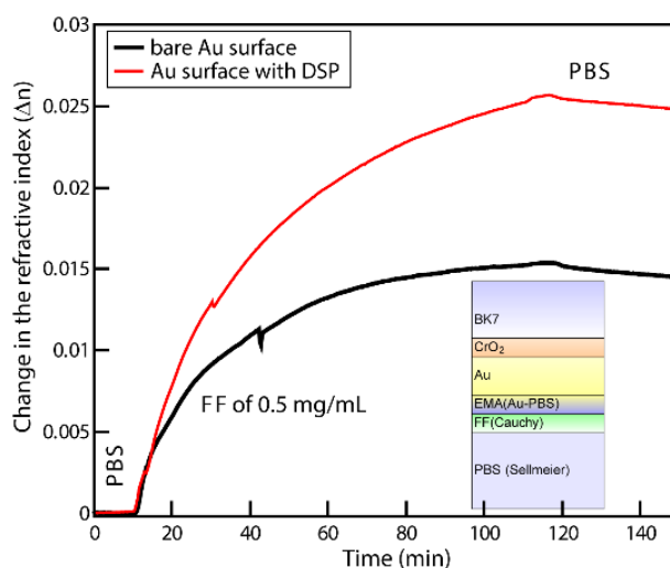
Figure 2: Increase of refractive index (at the wavelength of 633 nm) in the layer modelling the filaments at the interface during adsorption to gold surface with (red line) and without (black line) a DSP layer for covalent bonding. The change of refractive index corresponds to surface densities of 391 \text{ng}/\text{cm}^2 and 184 \text{ng}/\text{cm}^2 , for DSP-covered and non-covered surfaces, respectively.
