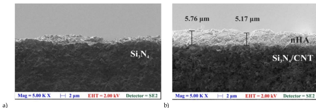
Figure 1: Electrospayed nHAP layer after 45-minute-long ESD process with the same deposition parameter a) \text{Si}_3\text{N}_4 , b) \text{Si}_3\text{N}_4/\text{MWCNT} substrates
