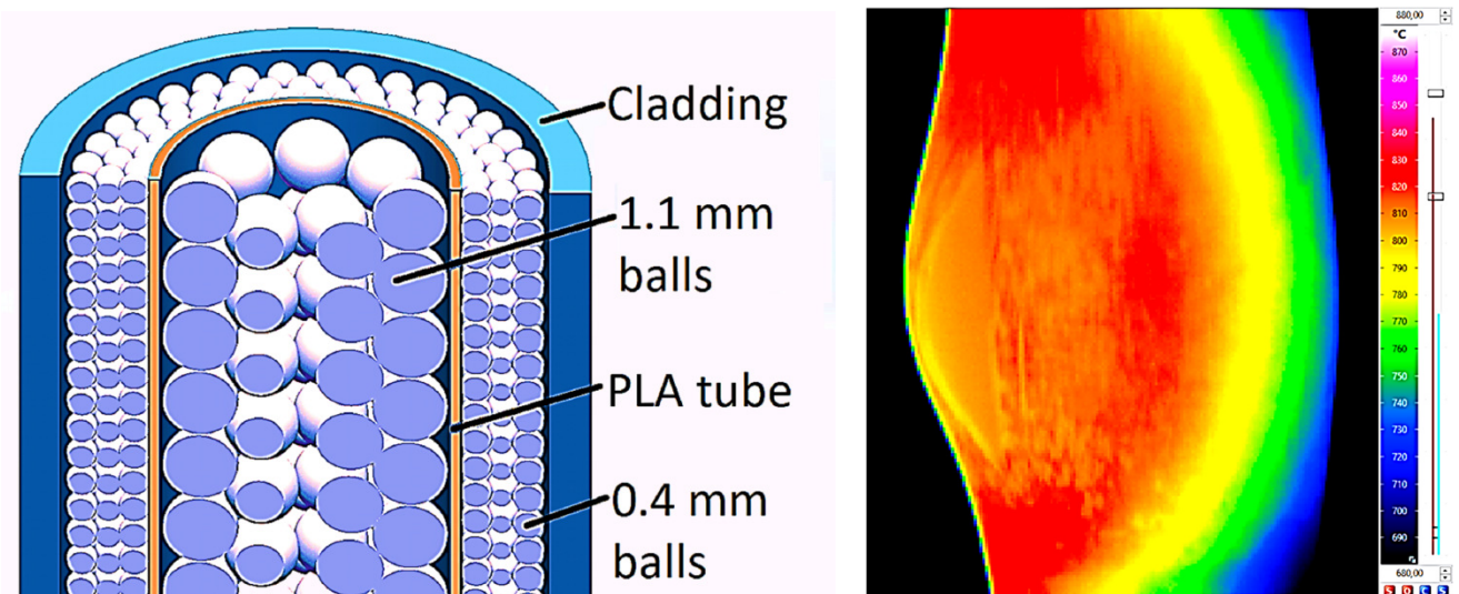
Figure 1: The model of the fragmented fuel pellet (left) and the infrared image of the cladding after burst (right).
