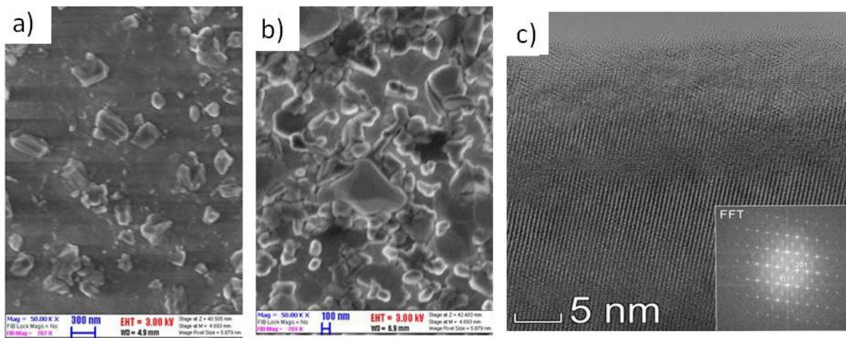
Figure 2: SEM image of the film after annealing in nitrogen (a), and oxygen (b) at 900°C for 3 hours, and the TEM image of the latter one
