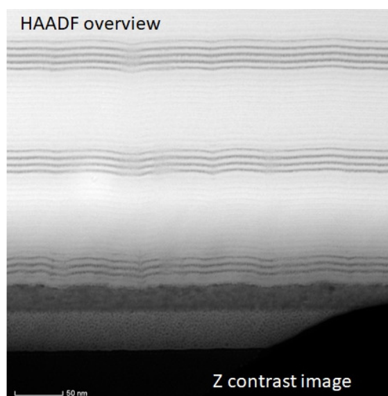
Figure 1: STEM-HAADF image of a WBC coating sputtered in an industrial chamber. The hierarchic multilayer structure, composed of \sim 5 nm layers, was formed due to the double rotation mechanism of the sample holder.
