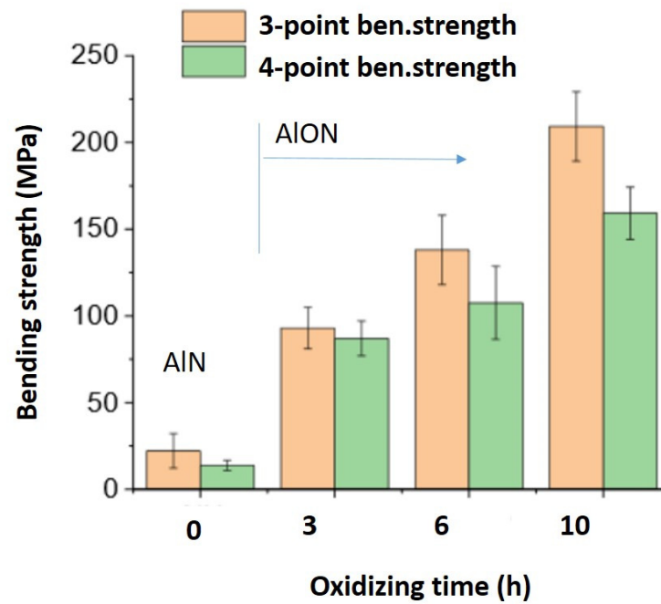
Figure 2: Bending strength of reference (AlN) and sintered AlON ceramics with different oxidation times
