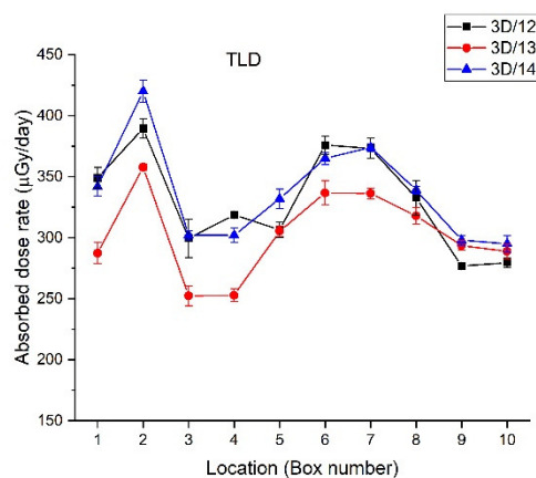
Figure 1: Absorbed dose rates measured by TLDs
