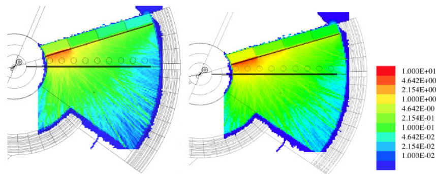
Figure 2: Simulated dose rate maps [ \mu\text{Sv/h} ] from the segmented axial wall made of Reference concrete. Simulations were performed with nominal (left) and recommended (right) initial concrete compositions.
