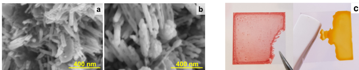
Figure 1: (a) SEM picture ( \times 100,000 ) of nano-arrayed \alpha\text{-Fe}_2\text{O}_3/\text{Ti} , (b) picture of the same surface after CPE in the presence of \text{Cu}(\text{II})/\text{H-GGG-OH} , in sodium borate electrolyte, at pH 9.2 [3] (c) typical drop-casted samples of 1 /ITO (red) and 2 /ITO (orange) [4].
