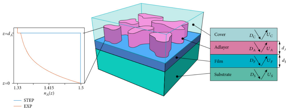
Figure 1: The structure of the modelled OWLS waveguide chips with inhomogeneous adlayer. The modelled multilayered assembly consists of four layers: substrate, waveguide film, adlayer, and cover.
