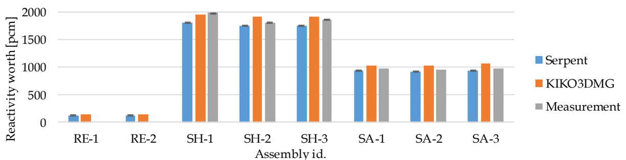
Figure 1: Calculation and measurement results of the regulating (RE), shim (SH) and safety (SA) sub-assembly reactivity worth in the CEFR
