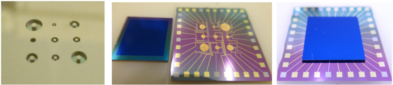
Figure 2: Processed test chip with nine force sensors of different lateral geometry. Force transferring rods in the handle wafer (left), 9x3 capacitors on the device layer side and the supplementary Si chip with a 1µm frame to prevent membrane deformation (centre) and test chip with back-side bonded deformation limiting Si element (right).
