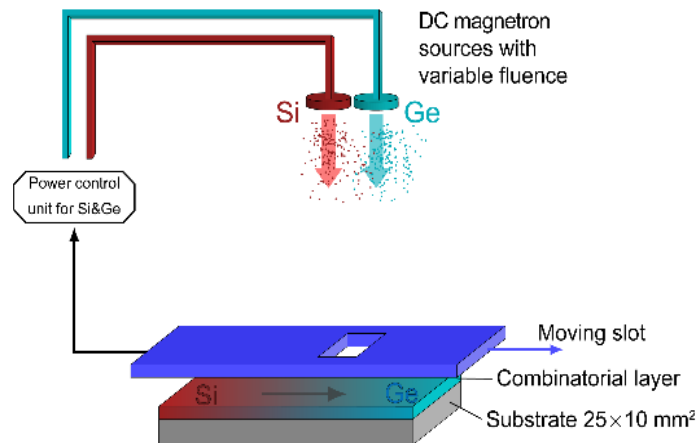
Figure 1: Setup used for the "single-sample concept" combinatorial deposition
