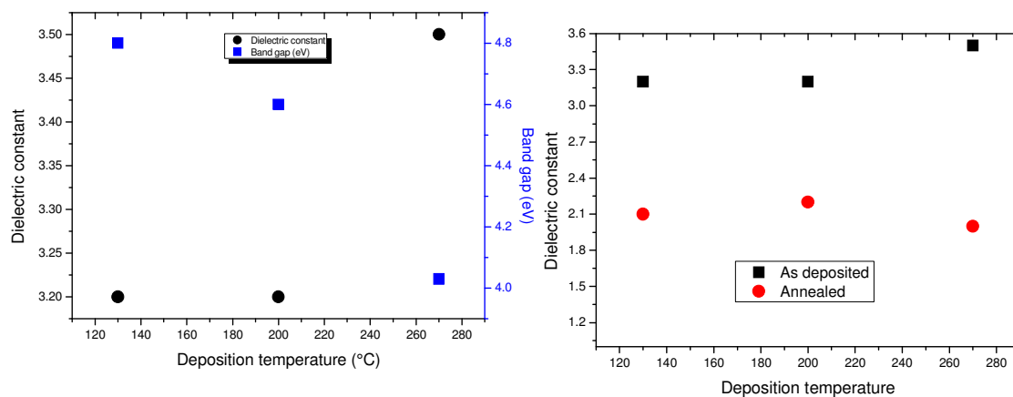
Figure 3: Dielectric constants and bandgaps of the as deposited and annealed films as determined by spectroscopic ellipsometry
