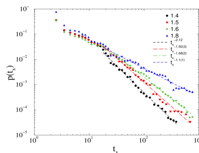
Figure 2: Duration distribution of on the KKI-18 model for growth K = 1.4 (bullets), 1.5 (boxes), 1.6 (diamonds), 1.8 (triangles). The dashed line shows power-law (PL) fits to the tail region: t_x > 20 .
