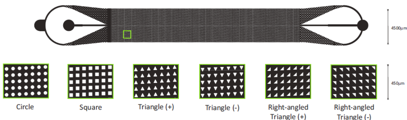
Figure 1: Layout and pillar types of the proposed DLD structure
