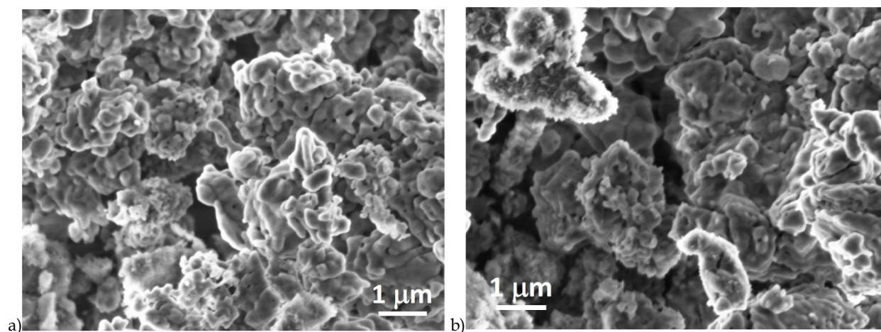
Figure 1: SEM image of oxidized AlN powder. a) 3 h, b) 10 h
