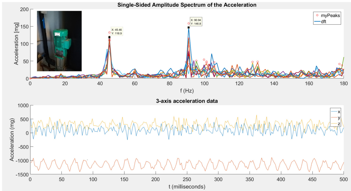
Figure 2: Vibration analyser measurement results on an air-ventilation pump, these results are essential to tune a piezoelectric cantilever for energy harvesting
