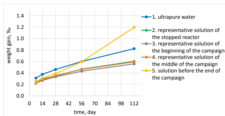
Figure 2: Weight gain of E110G samples treated in different solutions at 300 °C and 86 bar
