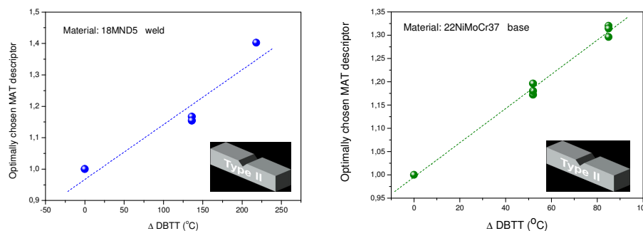
Figure 1: Selected MAT descriptor as a function of the transition temperature shift for the 22NiMoCr37 and 18MND5 materials
