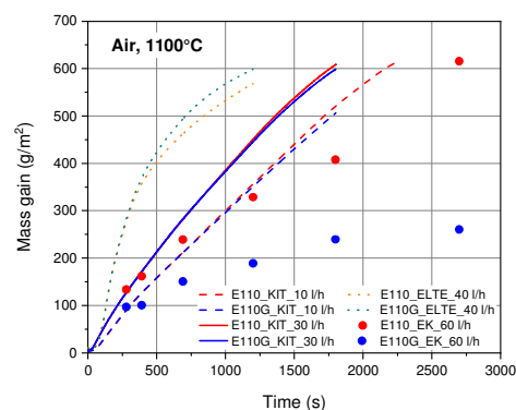
Figure 2: Comparison of mass gain of E110 and E110G tube segments oxidised in air at 1100 °C in different measurements
