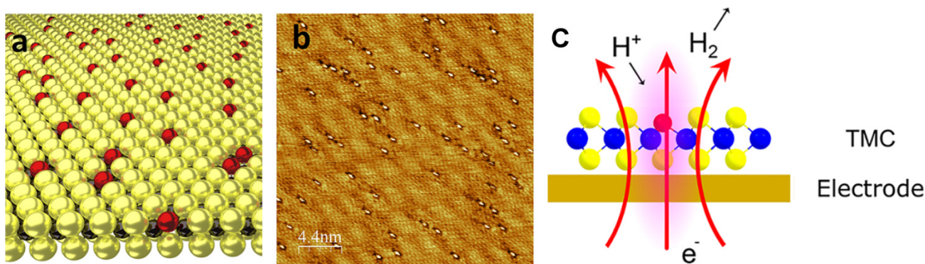
Figure 1: (a) Schematic model of individually dispersed heteroatoms substituting chalcogenide atoms of 2D transition metal chalcogenide crystals. (b) The practical realization of such structures evidenced by atomic resolution STM images of oxygen-atom-doped MoS 2 . (c) Schematic model of the hydrogen evolution reaction in the presence of the heteroatom.
