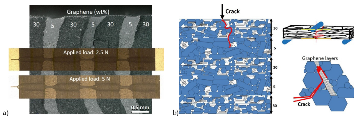
Figure 1: GMCS with seven multilayers. a) SEM image with depth profile, b) schematic view of the crack propagation mechanism in GMCS structure
