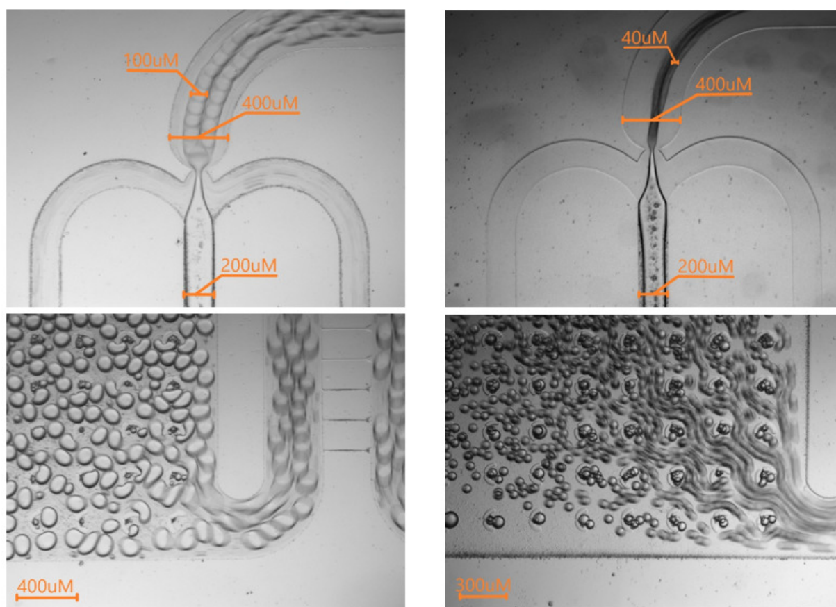
Figure 1: Droplet generation in junction type two-phase microfluidic system in case different flow rates of the dispersed (water) and continuous (oil) phase. The applied flow rates are: water – 0.1\mu\text{l/s} / oil – 0.3\mu\text{l/s} (left) and 0.4\mu\text{l/s} (right).
