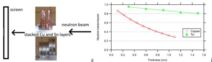
Figure 1: Arrangement of the Cu- and Sn-layers (a) and the determined neutron attenuations at different thicknesses (b)
