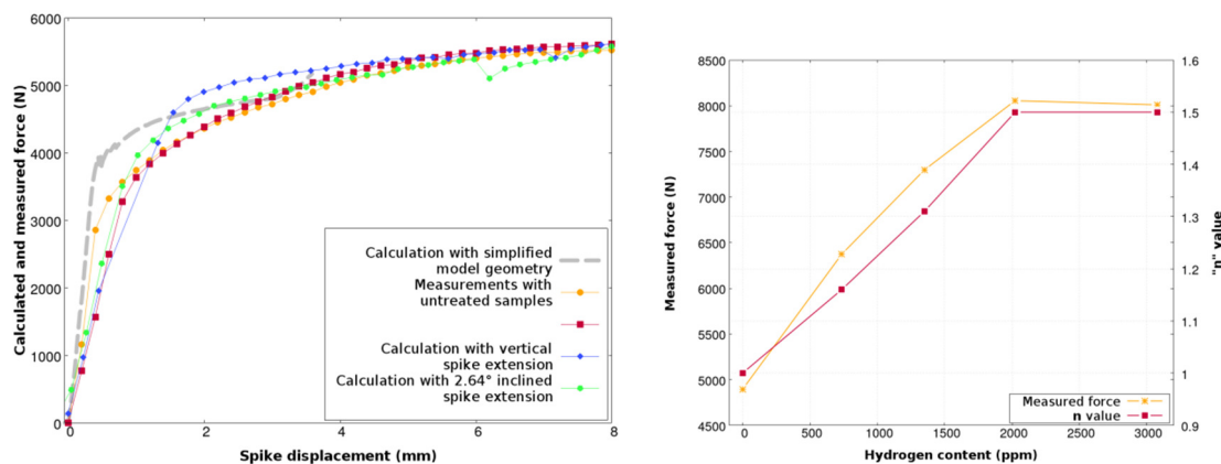
Figure 1: left figure shows calculated and measured stress strain equivalent curves, right figure shows the relationship between the maximum force and the "n" value.
