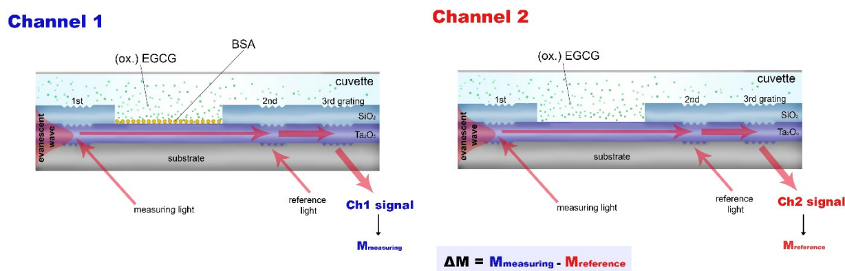
Figure 1: The sensor chips used in the WAVE instrument have two channels; one for measuring the interaction between the immobilized bioreceptor and the analyte (measuring channel, channel 1) and one for subtracting the channel 1 signal by a reference signal (reference channel, channel 2). In our case, BSA was immobilized on channel 1 surface, while channel 2 remained unmodified.
