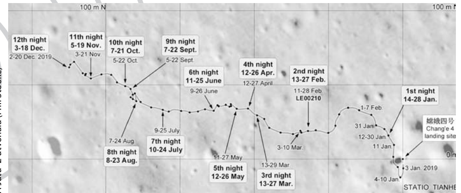
A Jütü-2 útvonala (Phil Stooke)
