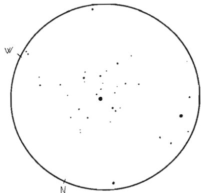
Collinder 419
