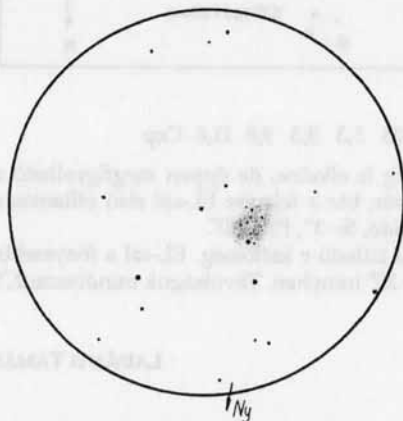
Berkeley 65
