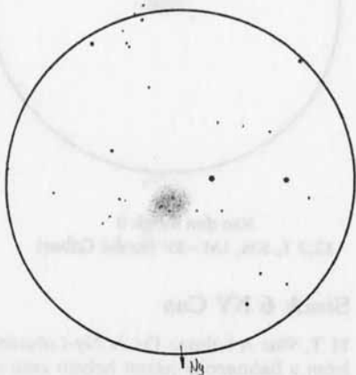
King 4
