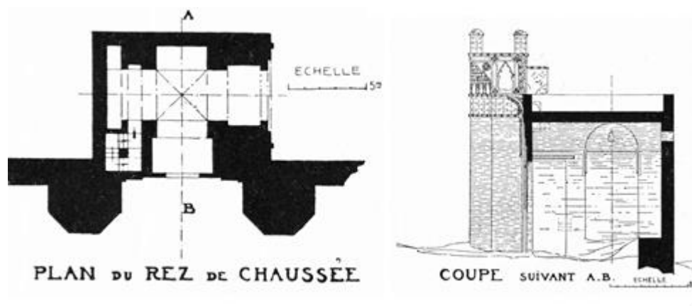
Fig. 5. Site plan and cross section of the main gate of Šālla, built in 1339.
