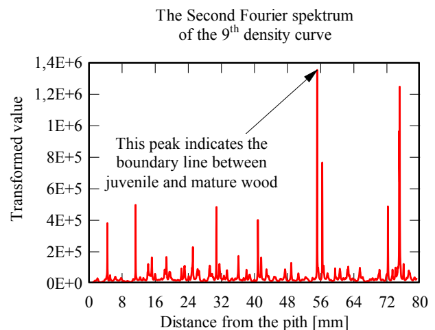
Figure 4 – 2 nd Fourier spectrum of density distribution of sample nr. 9.
