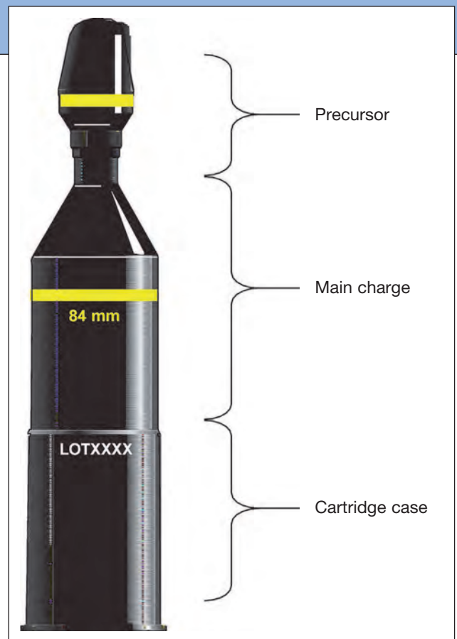
Figure 11. Structure of the HEAT 751 tandem-warhead ammunition
