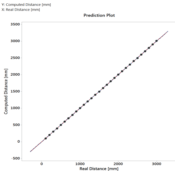
Fig. 8. The prediction plot, for the actual real distance and the distance computed, by the system using cameras.
