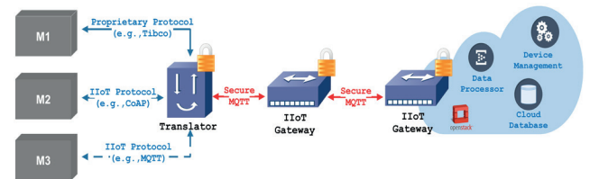
Fig. 5: CPPS end-to-end communication use case
