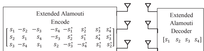
Fig. 2 Extended Alamouti Scheme for 3x3.
