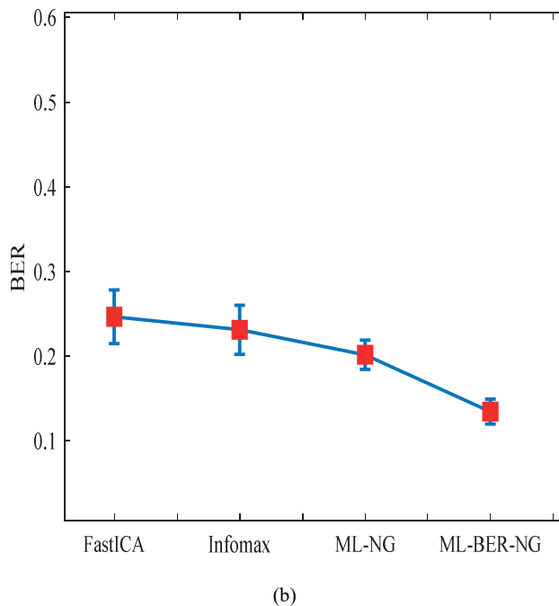
Fig. 5 BER performance comparisons of different representative methods
