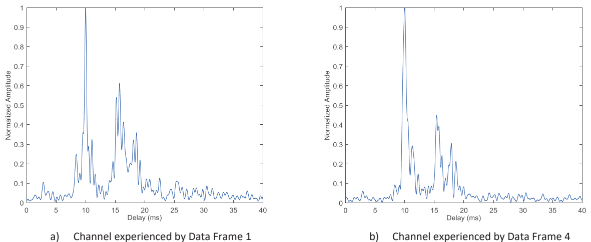
Figure 9: Measurement of CIRs in sea experiment
