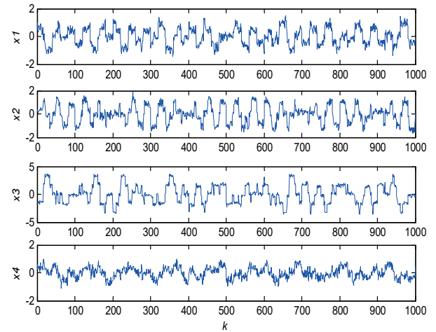
(b) Received mixed signals;
