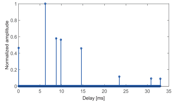
Figure 2: Simulated Channel Impulse response
