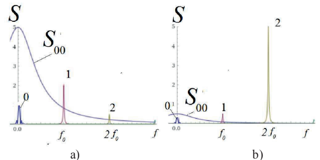
Figure 4. The spectrum structure (qualitative picture) of the PD photo-current of the OEO (Figure 1,c) at \varphi_{0MZ} = m\pi / 2 (a) and \varphi_{0MZ} = m\pi (b). Designations: DC component - 0, enlarged noise spectrum of DC component - S_{00} , fundamental harmonic - 1, second harmonic - 2
