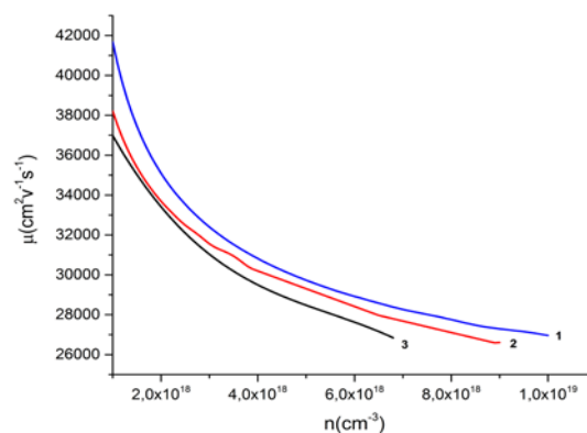
Figure 3. Calculated mobility due to scattering of electrons on impurity ions for electron concentration in the range of 10^{18} – 10^{19} cm -3 at temperatures: 1 – 300 K, 2 – 150 K and 3 – 77 K.
