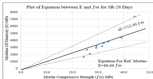
Figure 3. The plot of the equation between E and f_m for pond ash modified mortar for 7 and 28 days curing
