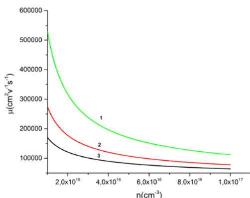
Figure 1. Calculated mobility due to scattering of electrons on impurity ions for electron concentration in the range of 10^{16} – 10^{17} cm -3 at temperatures: 1 – 300 K, 2 – 150 K and 3 – 77 K.
