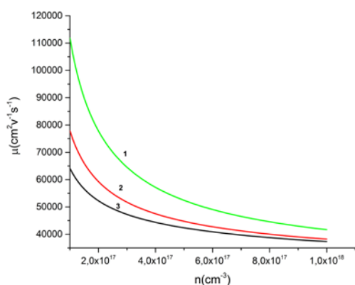
Figure 2. Calculated mobility due to scattering of electrons on impurity ions for electron concentration in the range of 10^{17} – 10^{18} cm -3 at temperatures: 1 – 300 K, 2 – 150 K and 3 – 77 K.
