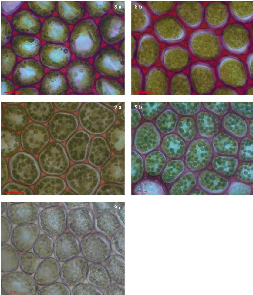
Photo 8a, b. P. platyphylla leaf cells at full turgor were frozen at a) -18^{\circ}\text{C} and b) -80^{\circ}\text{C} . After freezing neutral red staining was applied at pH 7.6. Scale bars = 2\ \mu\text{m} . Photo 9a, b, c. P. platyphylla leaf cells at full turgor were heated at a) 40^{\circ}\text{C} and b) 50^{\circ}\text{C} and c) 100^{\circ}\text{C} for 5 minutes. Before heating treatments neutral red staining was applied at pH 7.6. Scale bars = 2\ \mu\text{m} .
